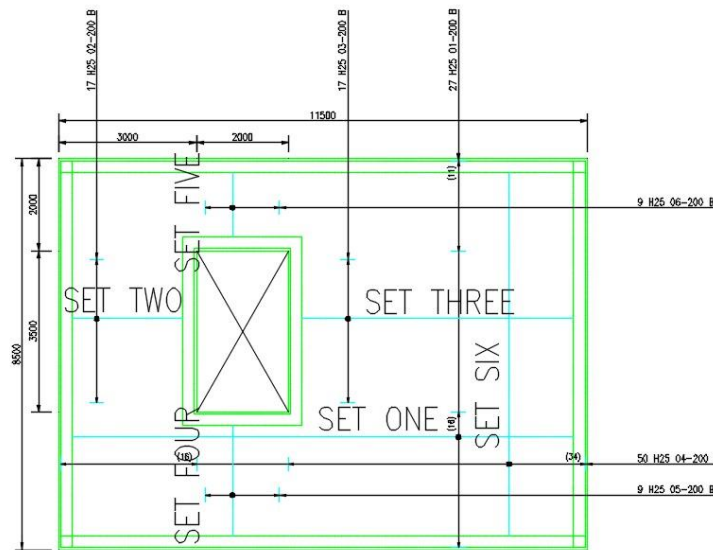
Figure 1.2.1:2 Reinforcement drawing showing bottom steel
