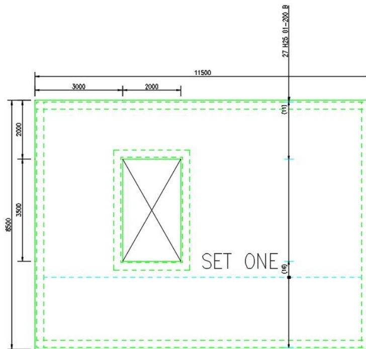
Figure 1.2.1:1 Slab with first set of bottom bar and range
