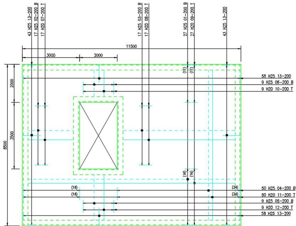
Figure 1.2.3:1 Reinforcement drawing showing top, bottom and side Steel
