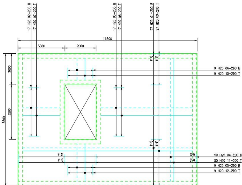
Figure 1.2.2:1 Reinforcement drawing showing the top and bottom Steel
