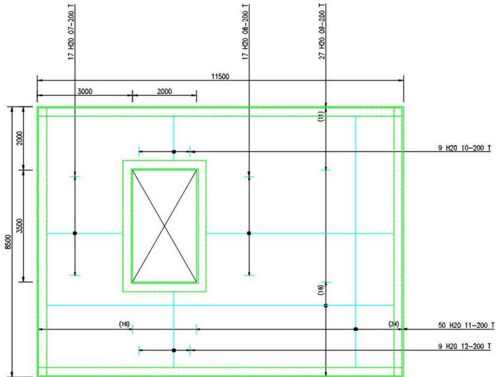
Figure 1.3.1:3 Drawing showing top steel only
