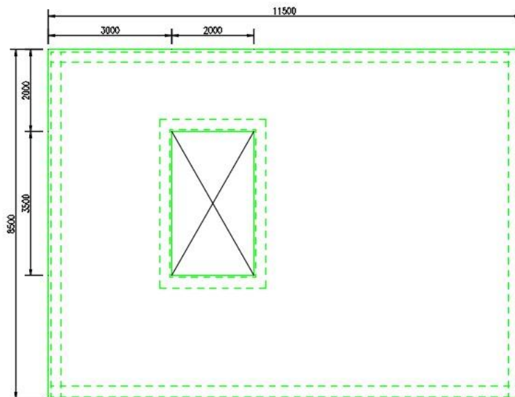
Figure 1.2:1 General arrangement drawing
