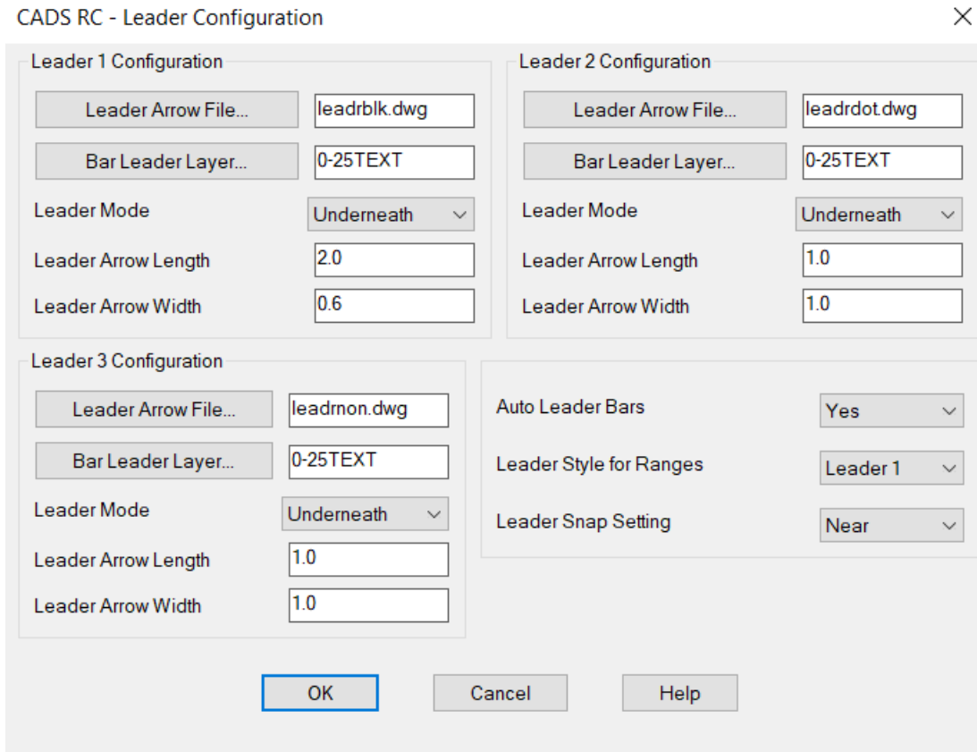
Figure 7.19.2.1:1 CADS RC Leader Configuration dialog
