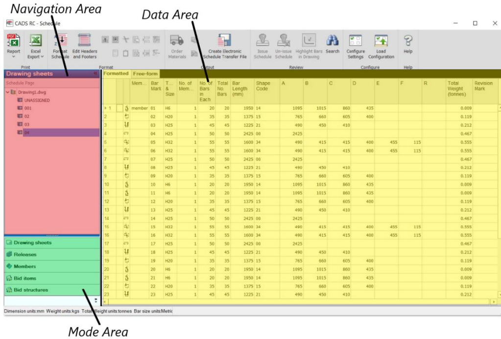
Figure 10.2:1 Schedule dialog
