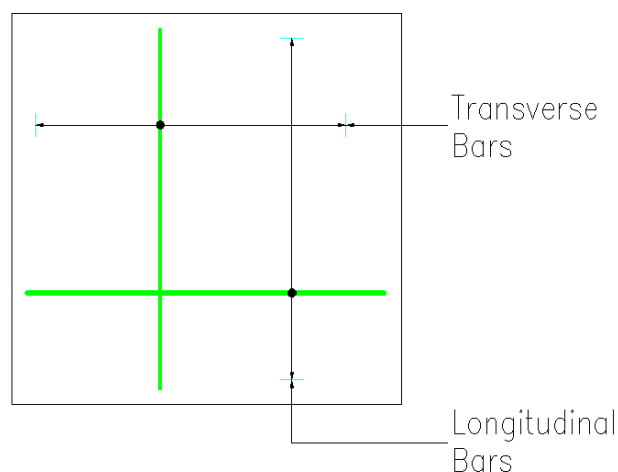
Figure 14.6.2:2 Bar Directions
