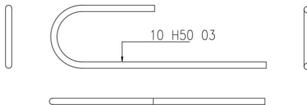
Creating a U Bar with a Semi-Circular Leg
