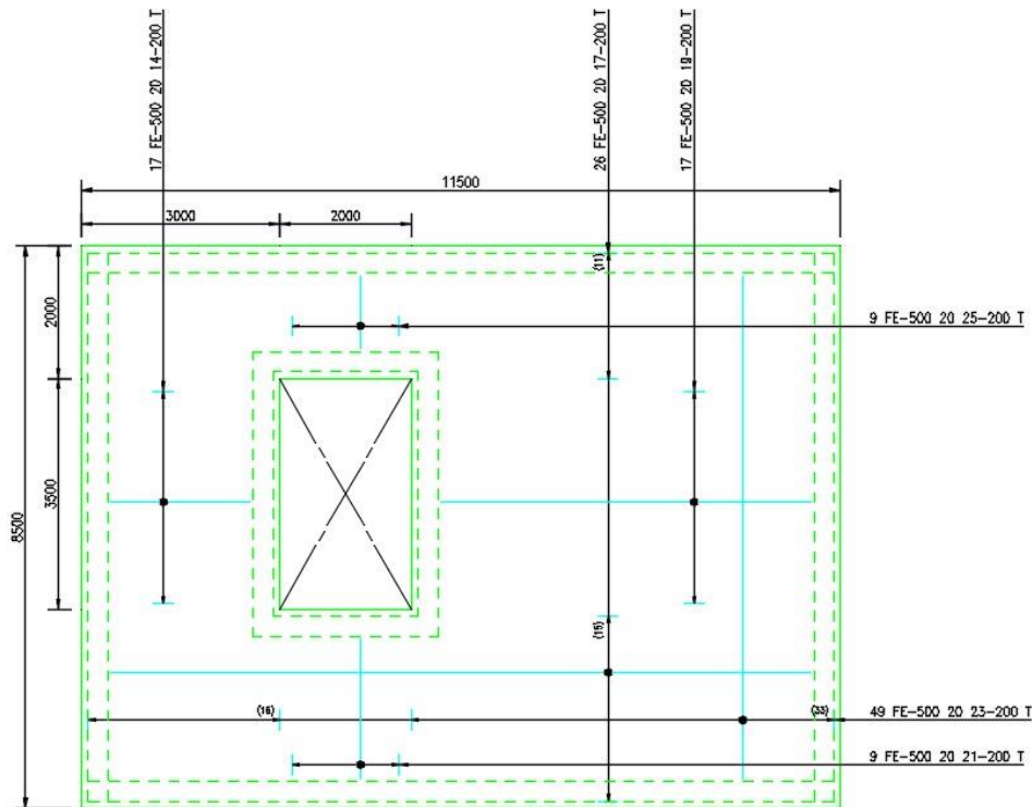
Figure 1.12 Drawing showing top steel only
