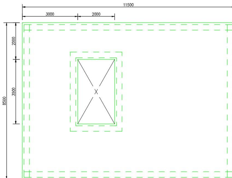
Figure 1.4 General arrangement drawing
