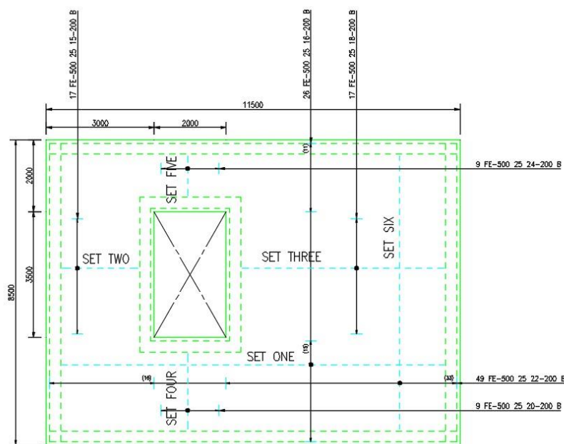
Figure 1.6 Reinforcement drawing showing bottom steel
