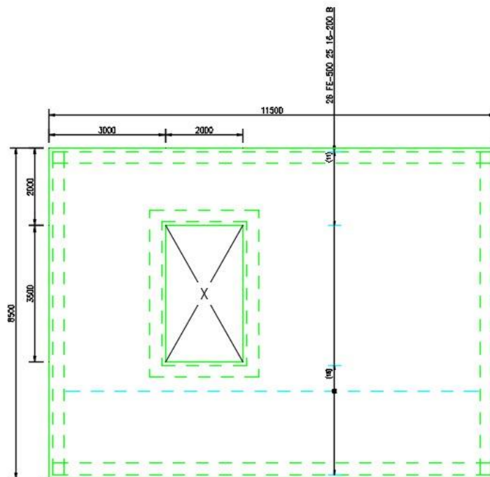
Figure 1.5 Slab with first set of bottom bar and range.
