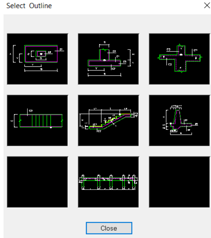
Figure 13.6.4:1 Outline dialog
