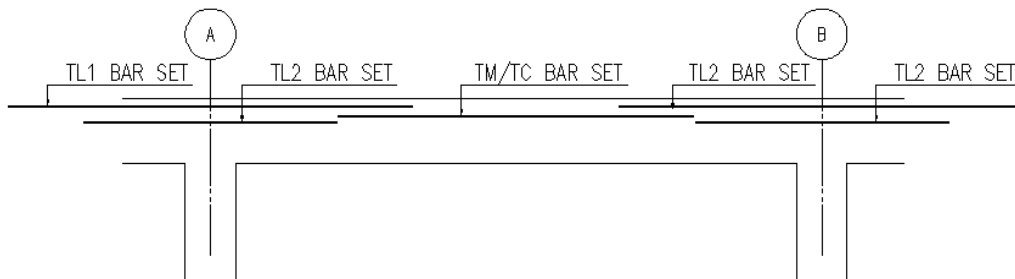
Figure 14.2.4:5 Top Bar Set annotation explained
