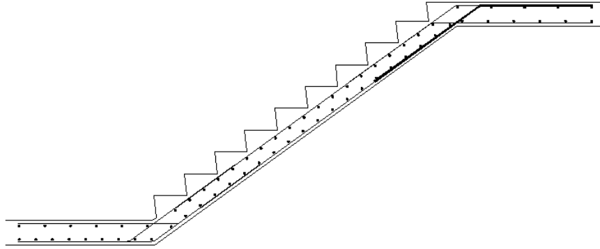
Figure 14.7.5:6 Bar Set 'F'
