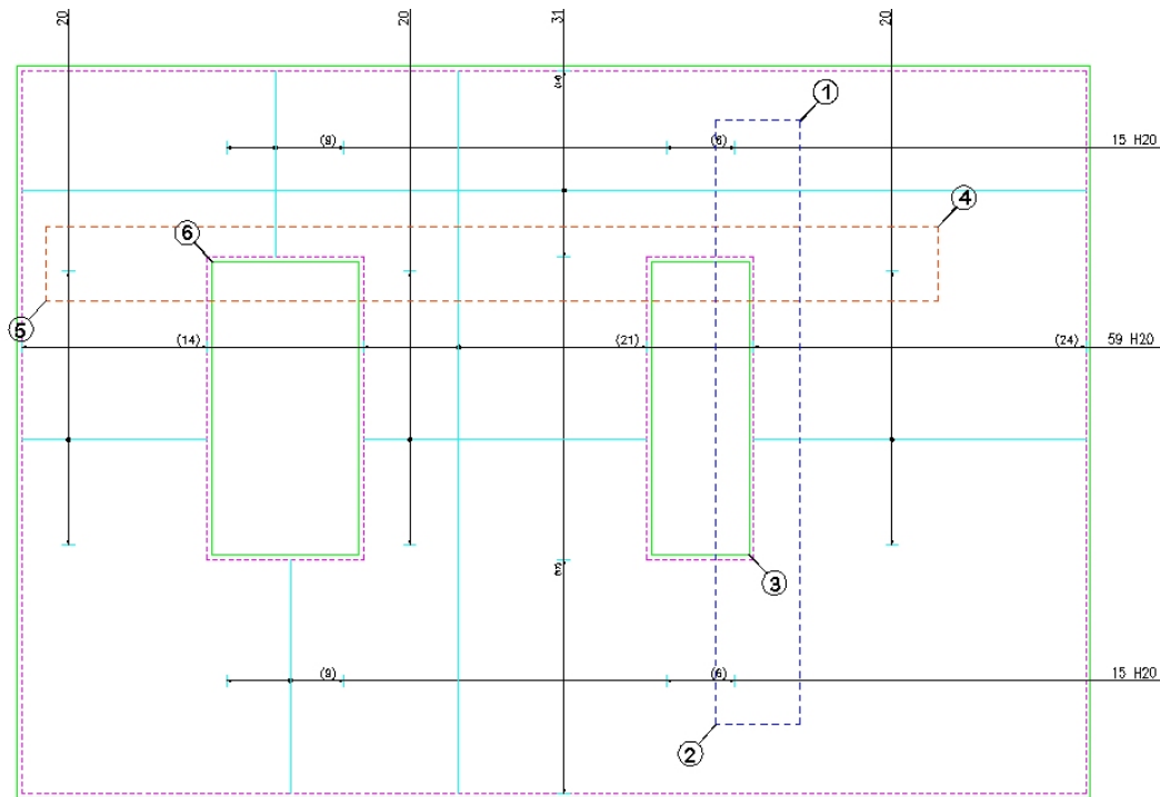
Figure 8.6.2:1 Slab with Opening to be resized
