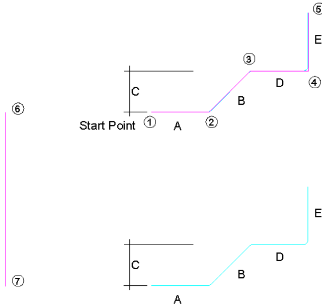
Figure 5.7.1:1 Creating a Shape Code 99
