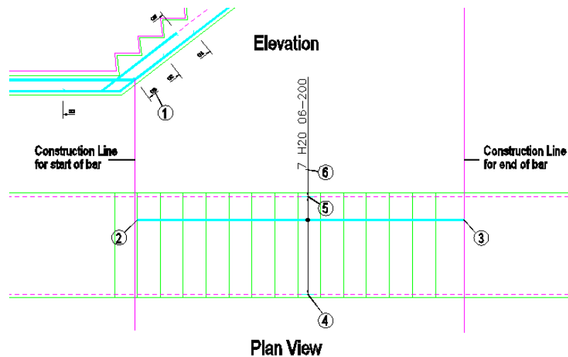
Figure 4.7.17:1 Use of Sketch Bar for projected view of Shape Code 00
