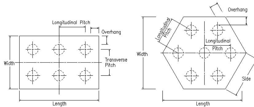
Figure 14.5.4:4 Six and Seven Pile Groups
