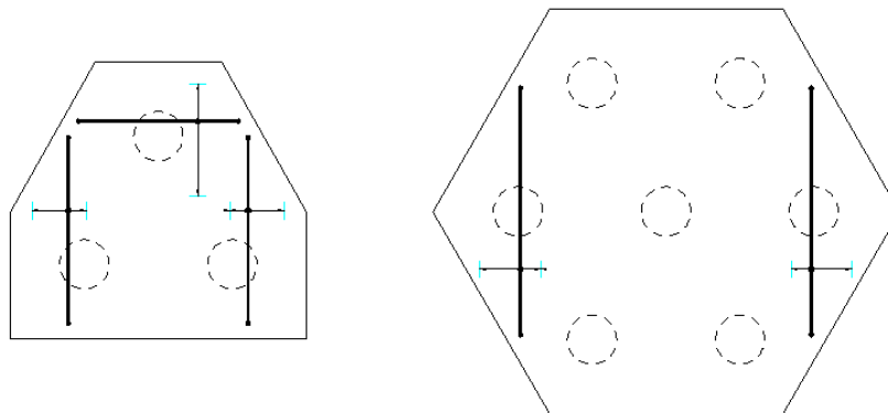
Figure 14.5.6:6 Three and Seven Pile, Secondary Reinforcement
