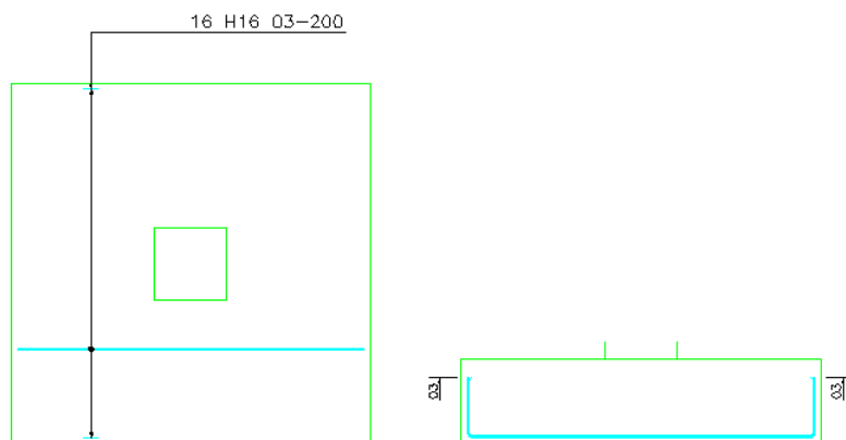
Figure 2.5:1 The bent bar drawn in section and plan
