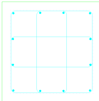
Figure 13.3.5:4 Typical Column Cross Section
