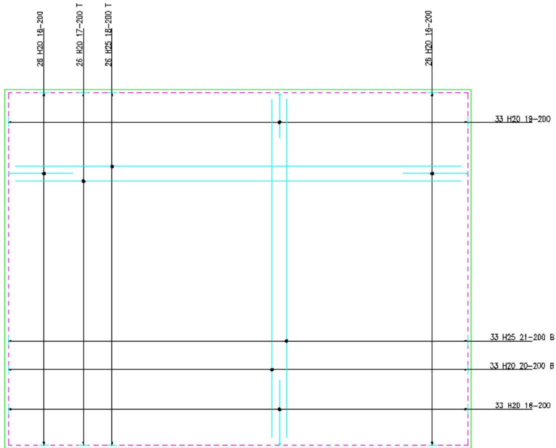
Figure 9.5.1:4 Drawing after Compact Bars have been run
