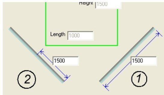
Figure 13.4.3:1 Trimmer Bar Lengths
