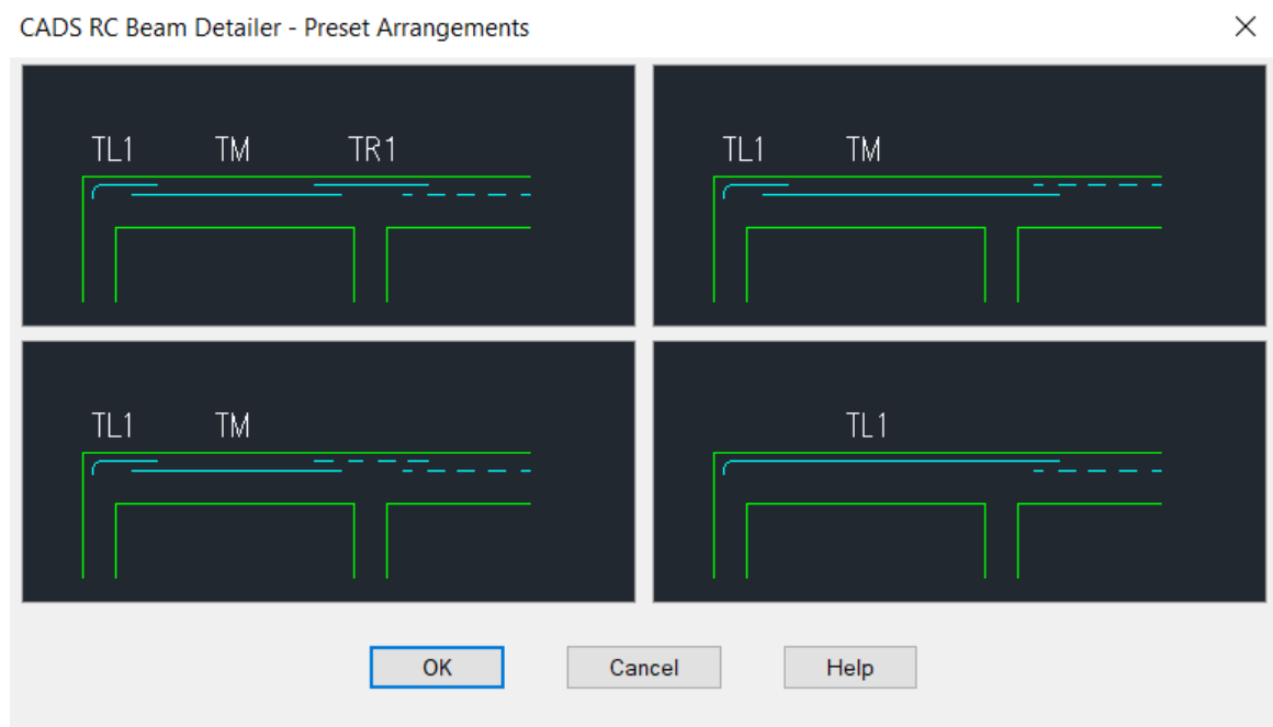
Figure 14.2.4:3 End Span Top Bar Pre-sets
