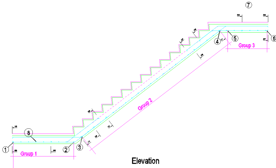
Figure 6.6.5:1 Adding Fixed Pitch Bar Run to Stair Elevation
