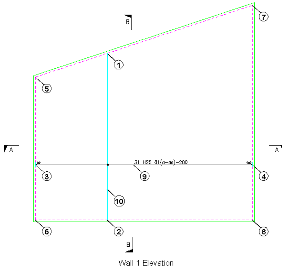
Figure 6.7.4:1 Adding a Linear Tapered Range to a Wall with one Tapered bar leg
