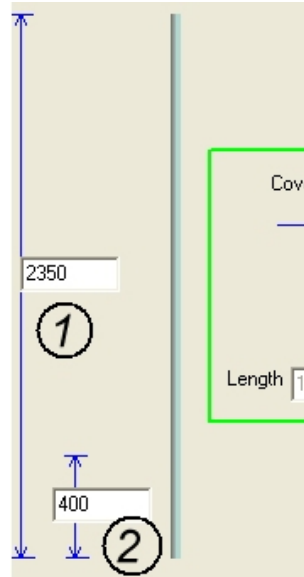
Figure 13.4.3:3 Left and right bar lengths
