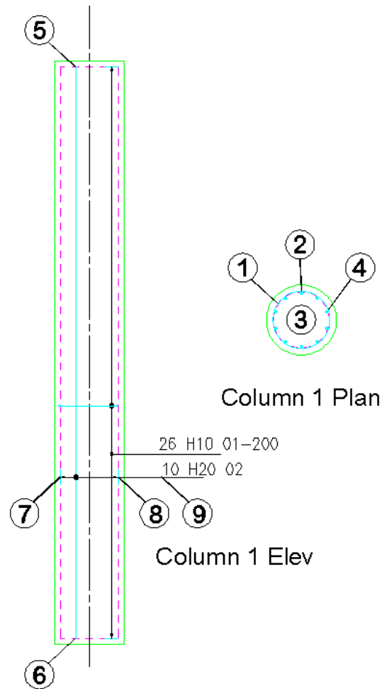
Figure 6.8.2:1 Adding Bars in Section using Run to Path to a Circular Column
