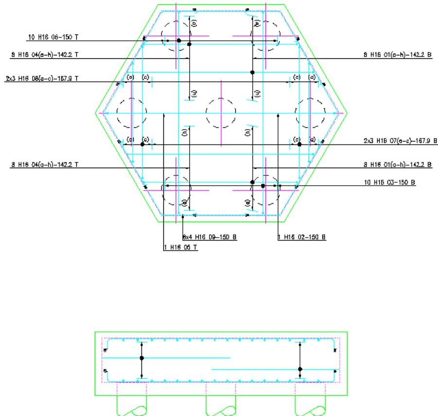
Figure 14.5.5:3 7 Group Pile Cap
