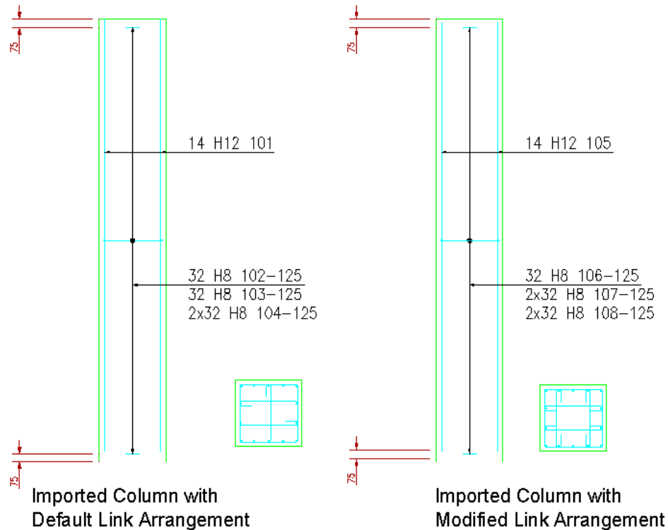
Figure 14.3.6:2 Typical Imported Column Details
