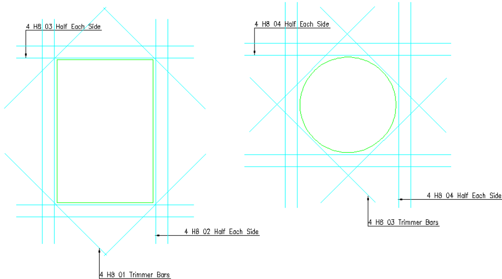
Typical Trimmed Opening Details
