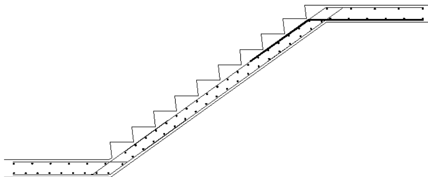
Figure 14.7.5:8 Bar Set 'H'
