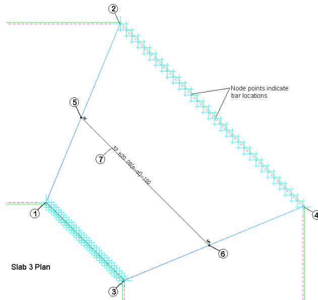
Figure 6.7.14:1 Adding a Trapezoidal Taper Range to a Floor Slab
