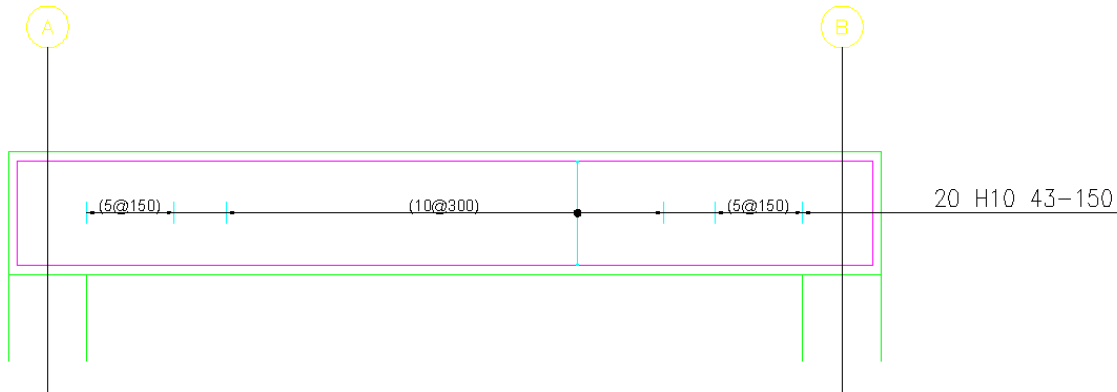
Figure 15.5.1:7 Finished Beam Detail
