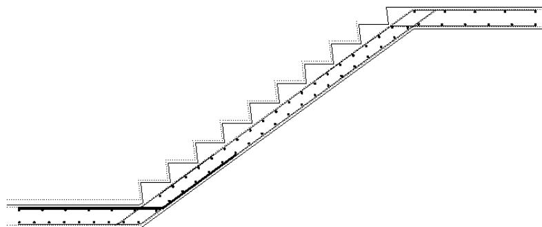
Figure 14.7.5:3 Bar Set 'C'
