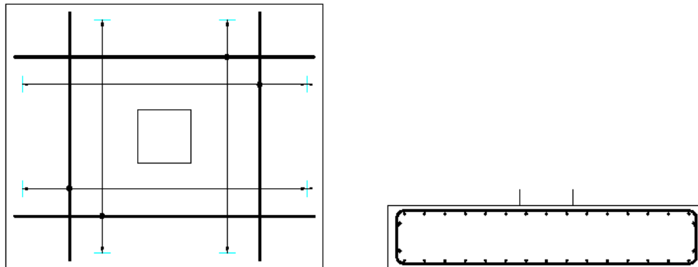
Figure 14.6.2:7 Typical Simple Bar Arrangement
