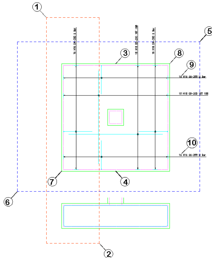
Figure 8.7.9:2 Completed detail using AutoCAD Mirror
