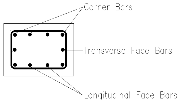
Figure 14.5.6:8 Pile Cap Column Bars
