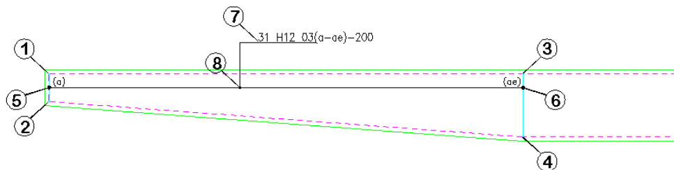
Beam 1 Elevation
