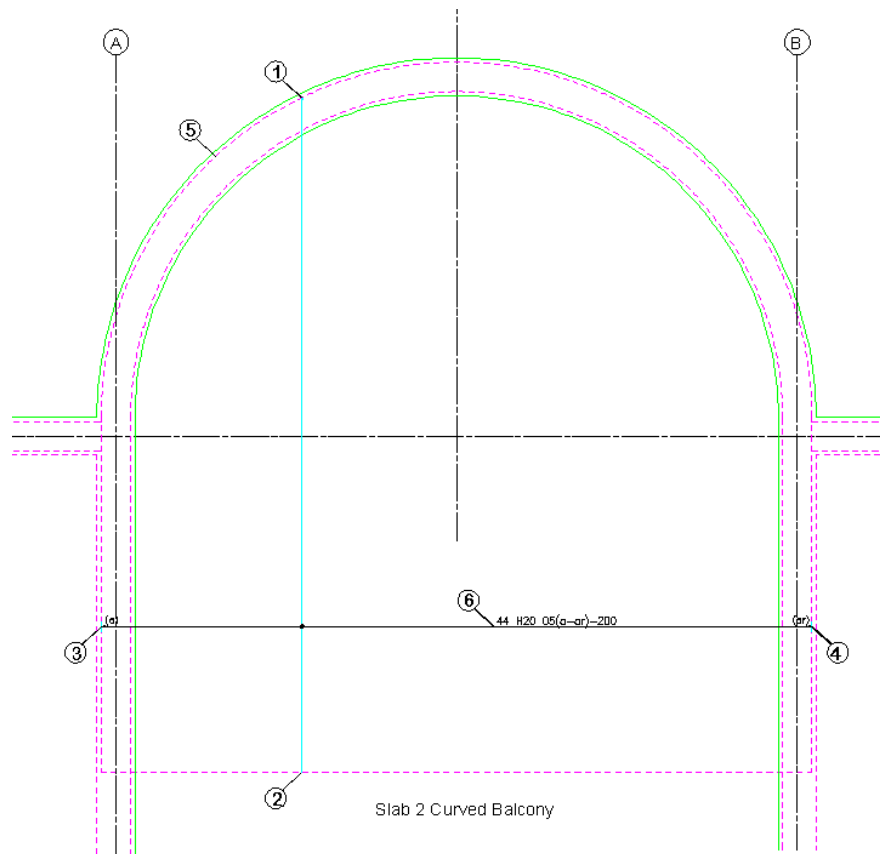
Figure 6.7.12:2 Adding a Varying Tapered Range to a Curved Balcony with two Tapered bar legs
