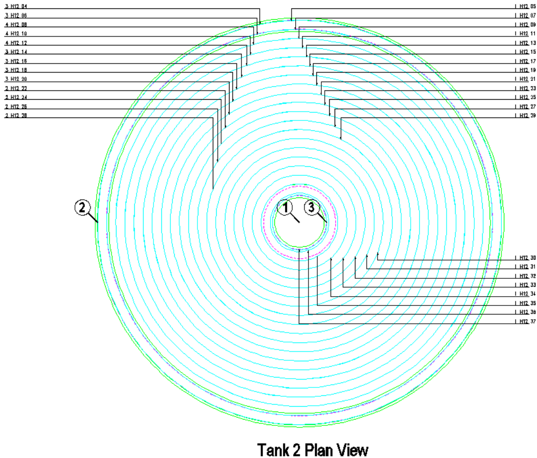
Figure 15.2.8:3 Finished Circular Bar Arrangement Detail
