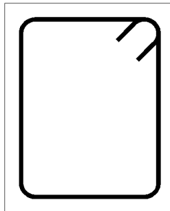
Figure 14.2.6:5 Outer Stirrup Bend Type
