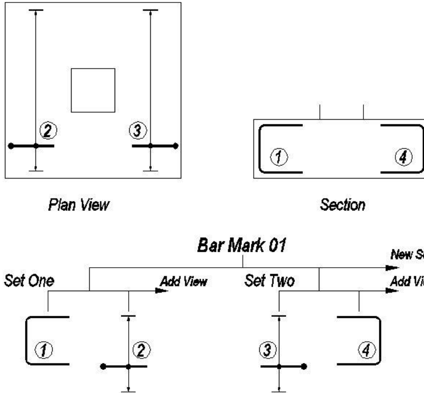
Figure 2.6.3:1 Illustrates a simple Pad Base with Bar Mark 01 shown within two ranges.
