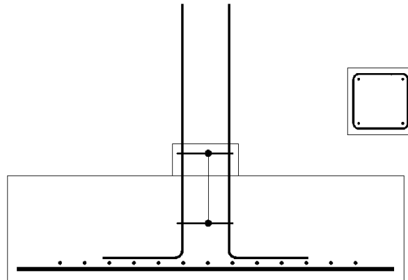
Figure 14.6.2:10 Typical Starter Bar Detail
