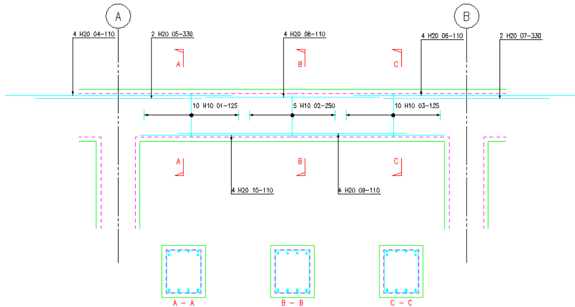
Figure 14.2.7:1 Typical Beam Detail and Sections
