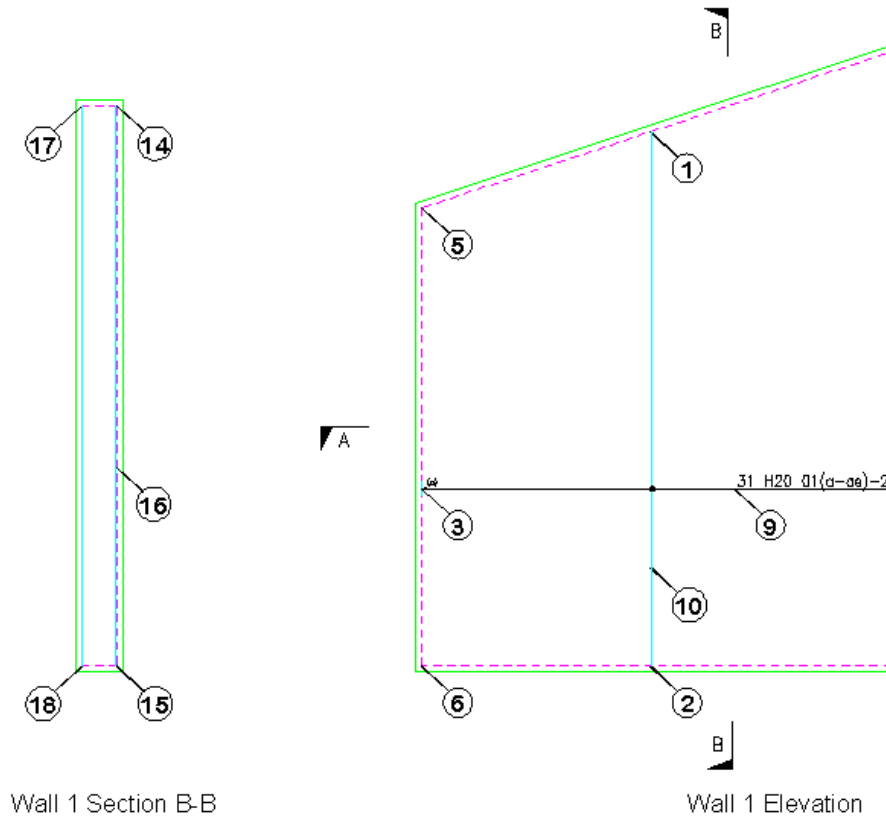
Figure 6.7.4:4 Adding Sketch Bar Views of the Linear Taper to the Wall Section
