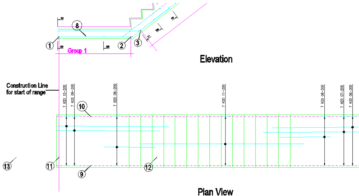
Figure 6.6.5:2 Adding the Fixed Pitch Range to the Stair Plan
