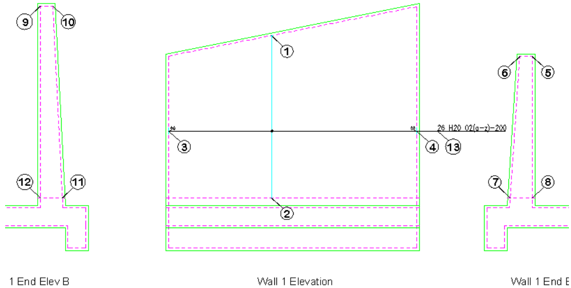
Figure 6.7.5:1 Adding a Linear Taper Range to a Wall with two Tapered bar legs
