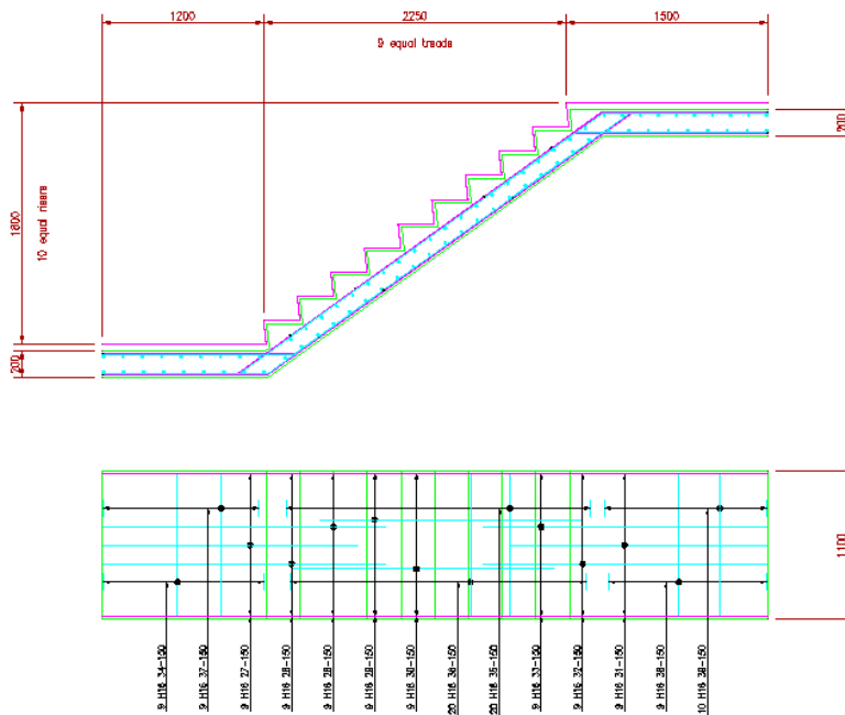
Figure 14.7.7:1 Typical Stair Flight Detail
