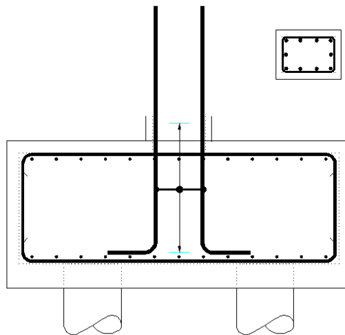
Figure 14.5.6:10 Typical Starter Detail
