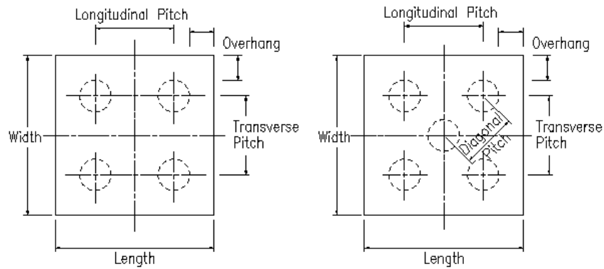
Figure 14.5.4:3 Four and Five Pile Groups
