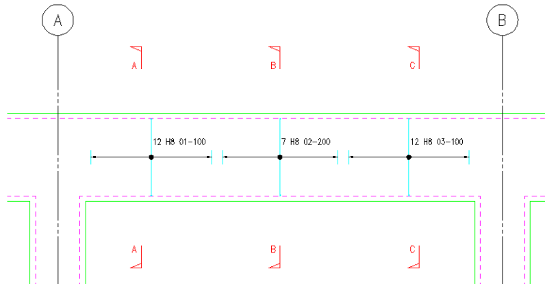
Figure 14.2.6:3 Beam showing Three Stirrup Zone
