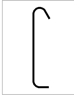
Figure 14.2.6:8 Inner Open Stirrup Bend Type
