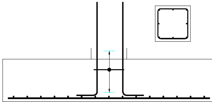
Figure 14.6.5:2 Typical Rectangular Column Starter Bar Detail
