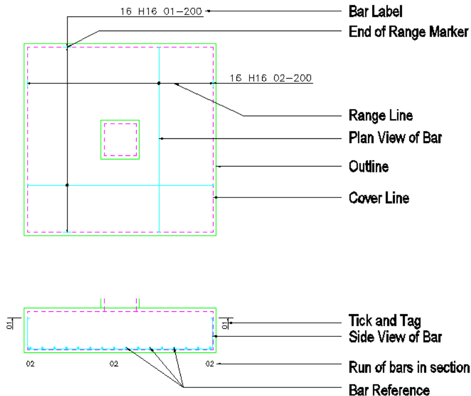
Figure 2.3:1 This is a drawing of a simple Pad Base with bottom reinforcement detailed.
