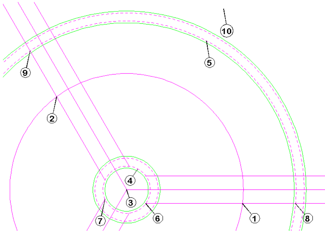
Figure 6.7.6:1 Setting Out points for Linear Taper
