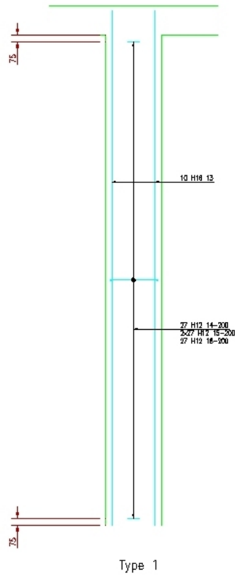
Figure 14.3.3:1 Column without column above
