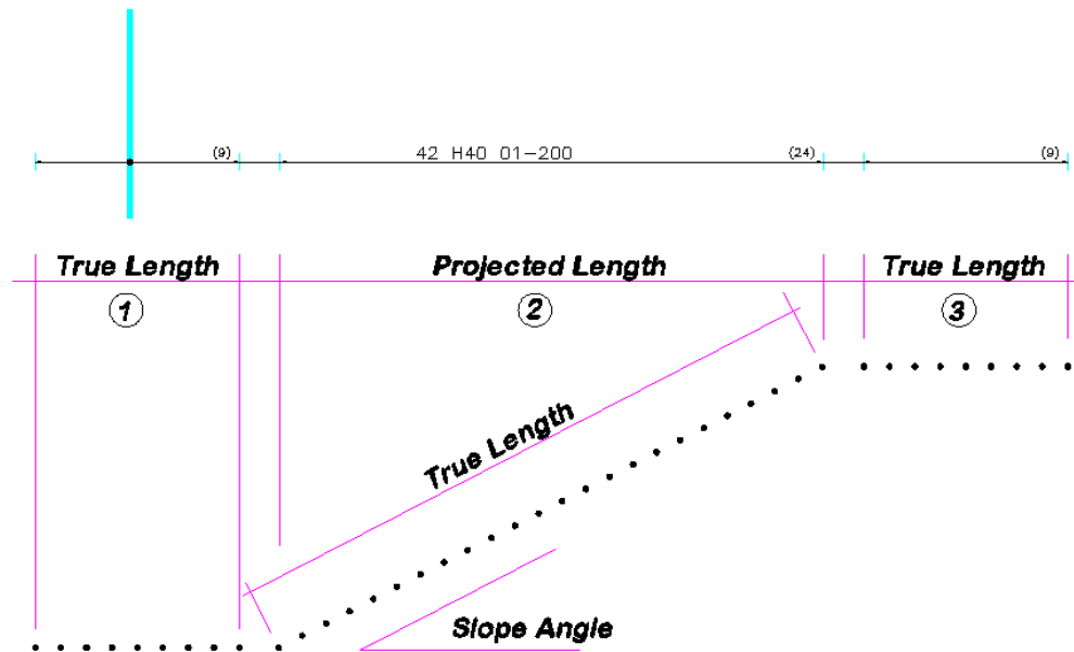
Figure 6.6:1 Section View of distribution steel on a staircase
