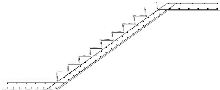
Figure 14.7.5:11 Bar Set 'K'
