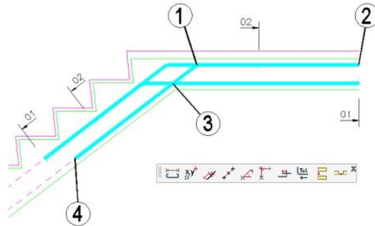
Figure 4.7.16:1 Placing Order of Shape Code 15 in the top landing
