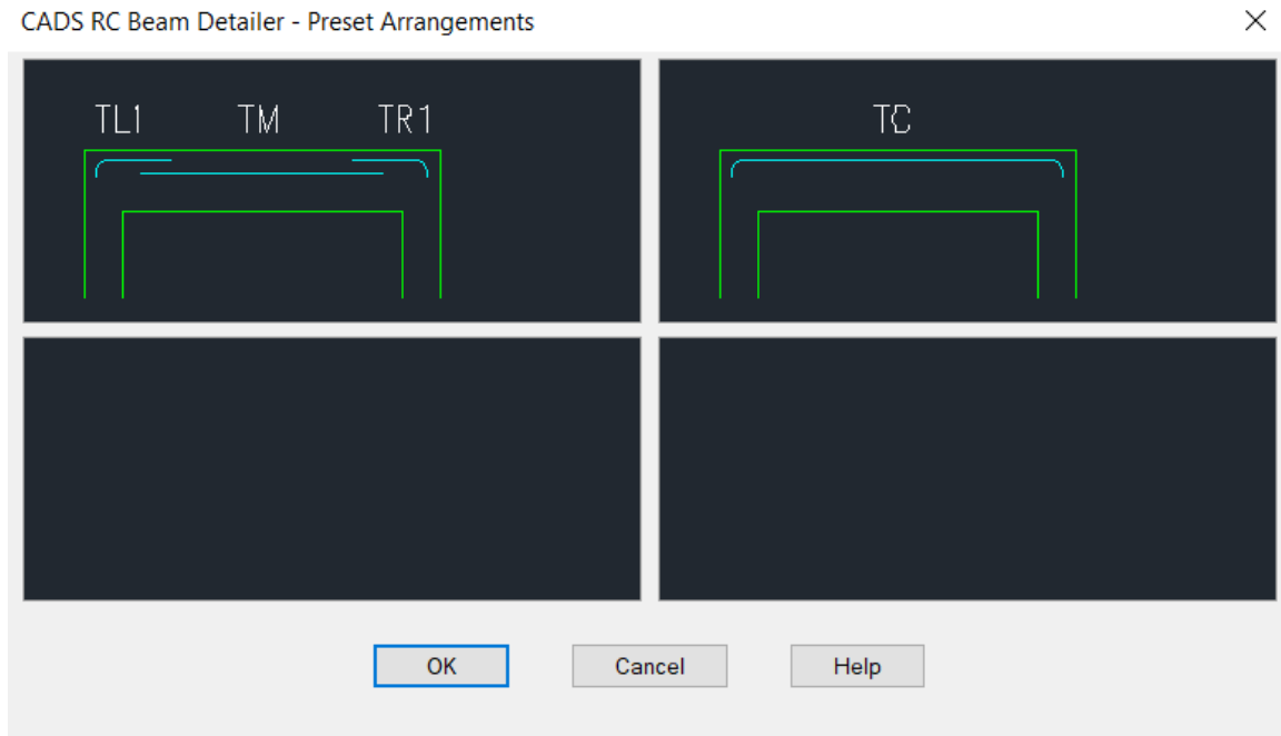
Figure 14.2.4:2 Single Span Top Bar Pre-sets
