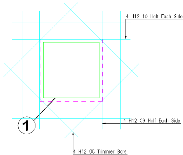
Figure 13.4.5:2 Finished Square Opening
