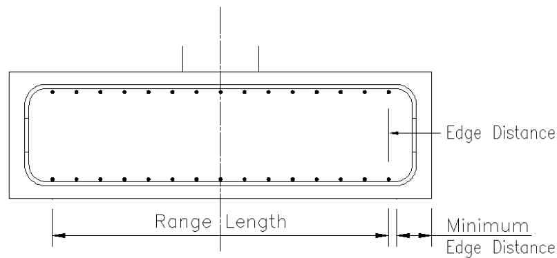
Figure 14.6.4:2 Edge Distance and Range Length
