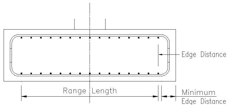
Figure 14.6.1:2 Edge Distance Information
