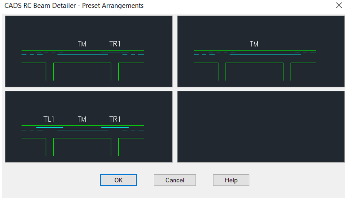
Figure 14.2.4:4 Interior Span Top Bar Pre-sets
