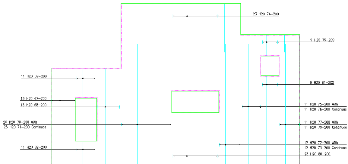
Typical 15.3.8:1 Typical Outline detailed with the Area Detailer
