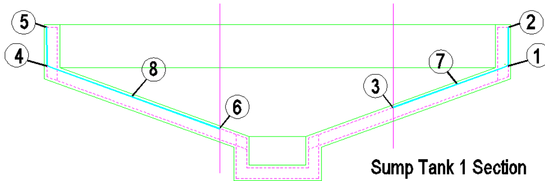
Figure 6.5.2:1 Adding two Shape Code 15's as different Bar Marks
