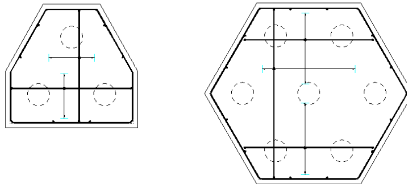
Figure 14.5.6:4 Main Reinforcement Bands
