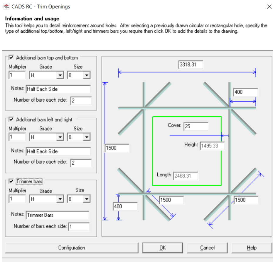
Figure 13.4:1 Trim Openings – Rectangular Opening
