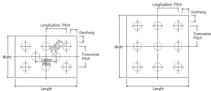
Figure 14.5.4:5 Eight and Nine Pile group
