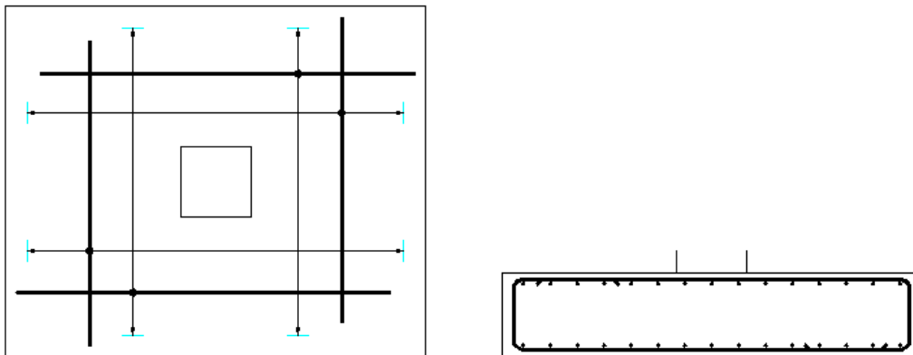
Figure 14.6.2:6 Typical Trombone Bar Arrangement
