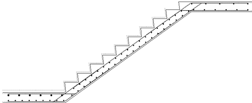
Figure 14.7.5:12 Bar Set 'L'
