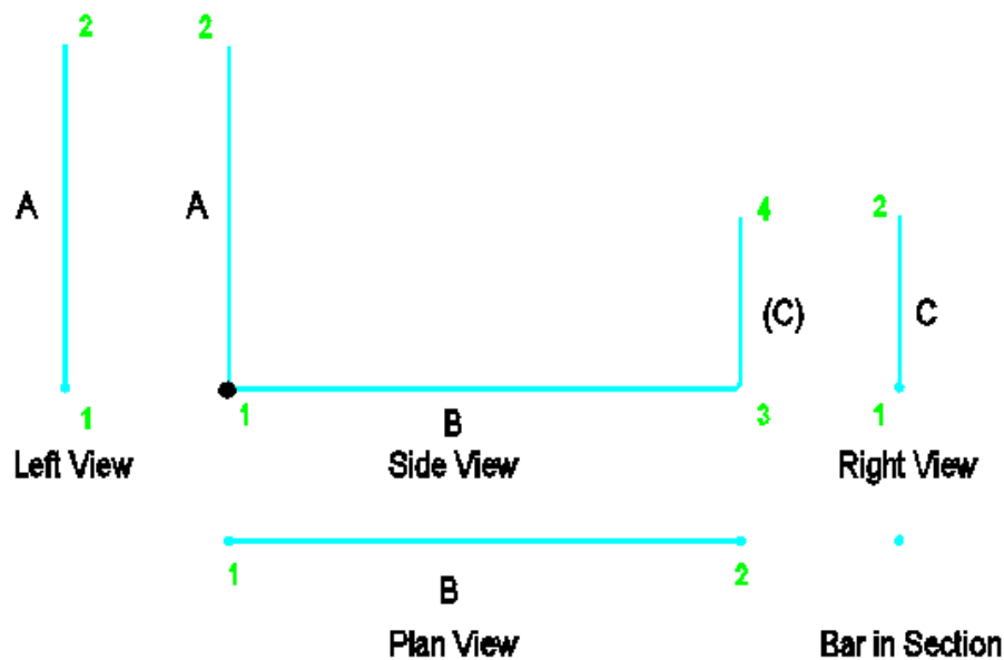
Figure 2.7:1 Bar Views with Placement point order
