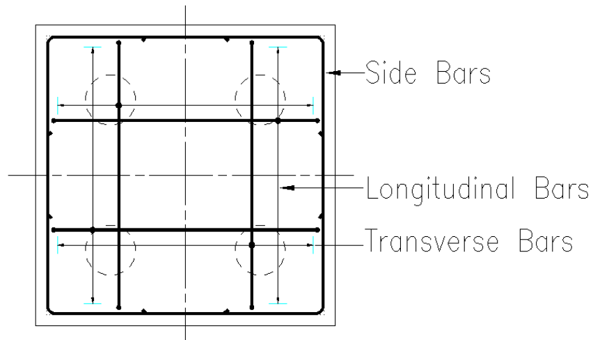
Figure 14.5.6:2 Typical Pile Cap Bar Sets
