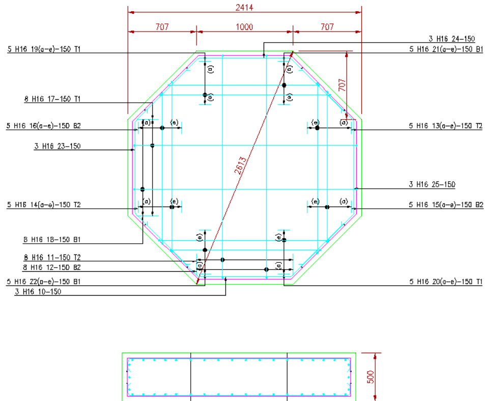
Figure 14.8.4:1 Typical Octagonal Pile Cap Reinforcement Drawing
