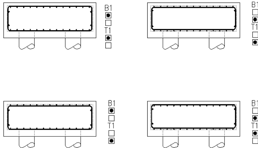
Figure 14.5.6:3 Bar Layering Options
