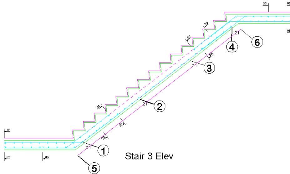
Figure 7.17.5:1 Bar References added to Staircase Elevation
