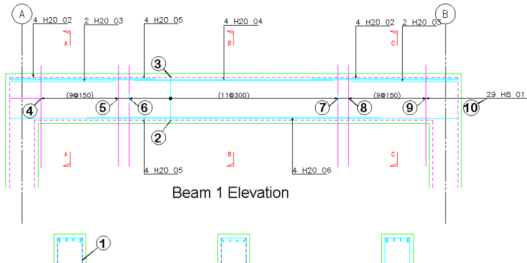
Figure 6.6.4:1 Adding a Single Multiple Pitch Range to a Beam Elevation
