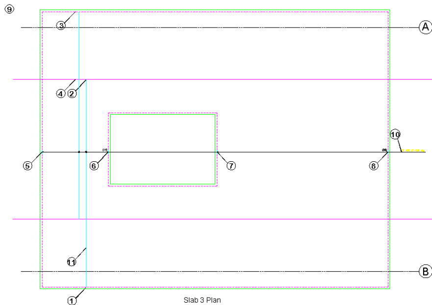
Figure 6.6.10:1 Adding a Staggered Fixed Pitch Range to a Floor Slab
