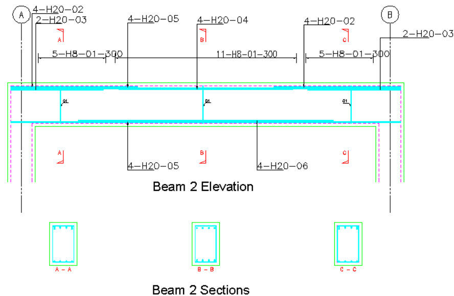
Figure 8.5.1:3 Results of Reconfiguring shown on Beam
