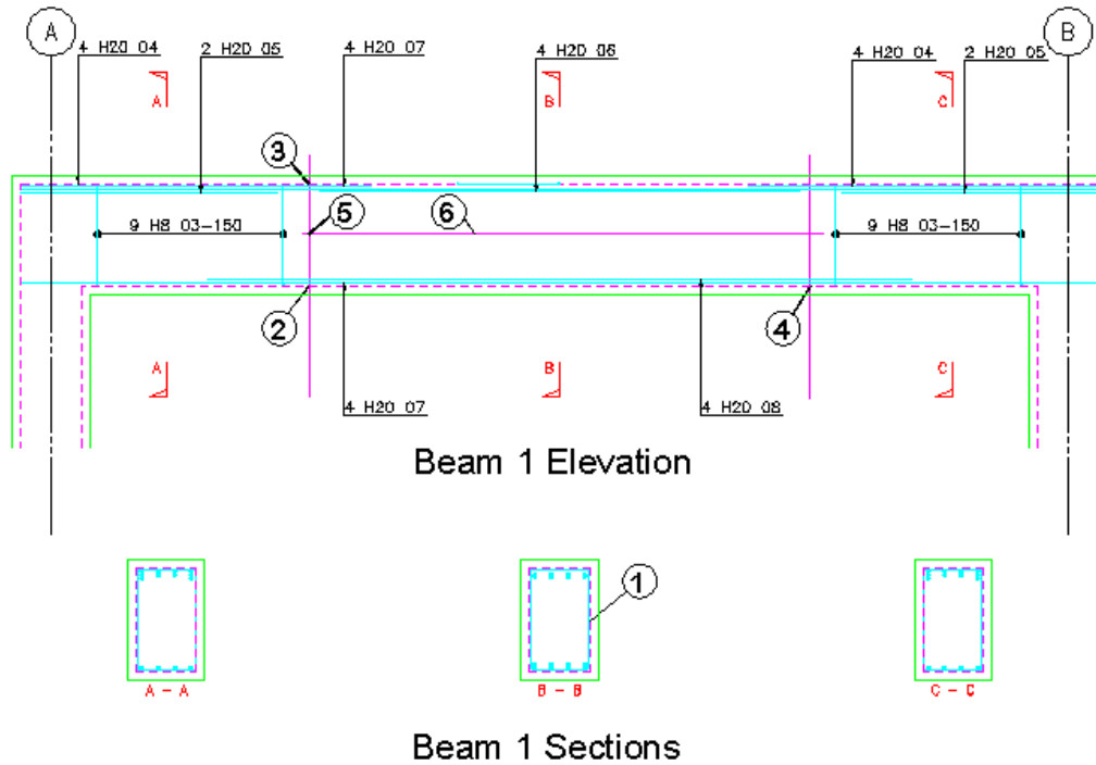
Figure 6.3.4:1 Adding a Double Indicator Range to the Beam Elevation
