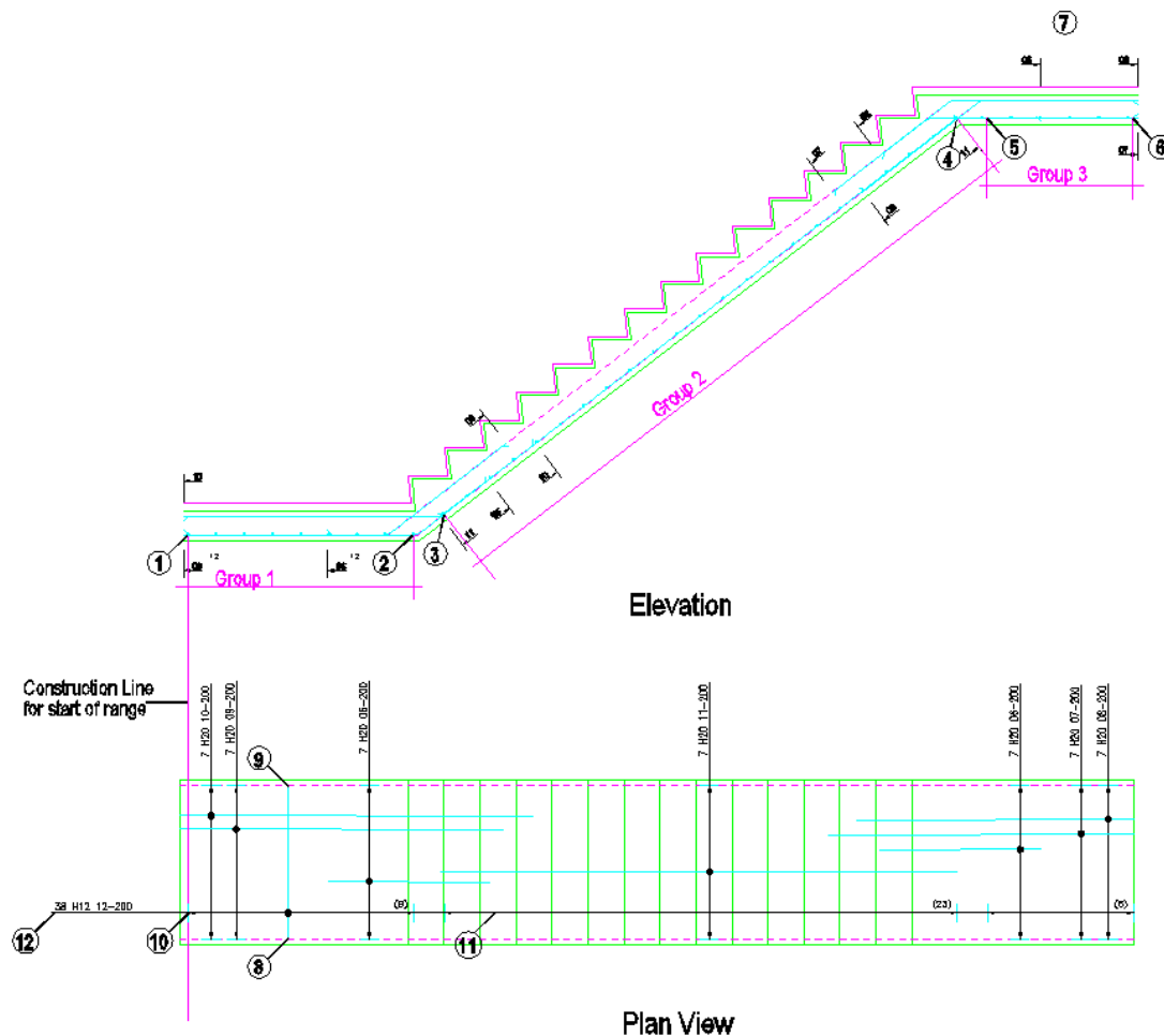
Figure 6.6.5:3 Fixed Pitch Range and Bars in Section added to Stair
