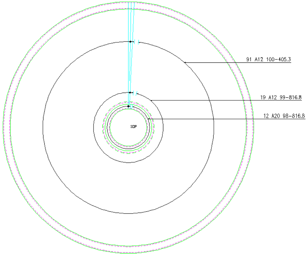
Figure 15.8.3:1 Radial Bars added to outline
