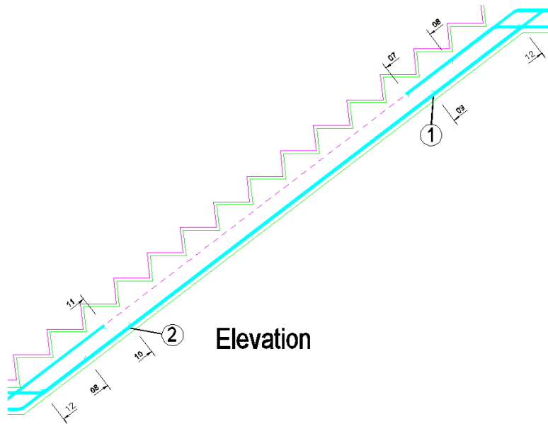
Figure 4.7.19:1 Lapping Bars on Staircase
