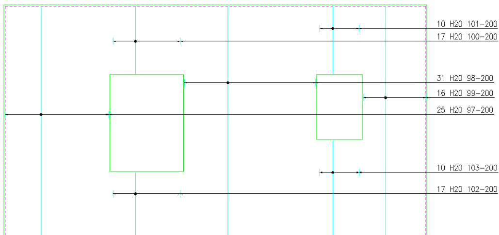
Figure 15.4:2 Finished Split Range Detail
