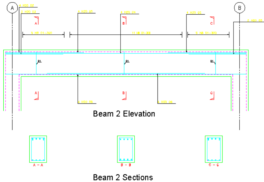
Figure 8.5.1:1 Beam before reconfiguring CADS RC
