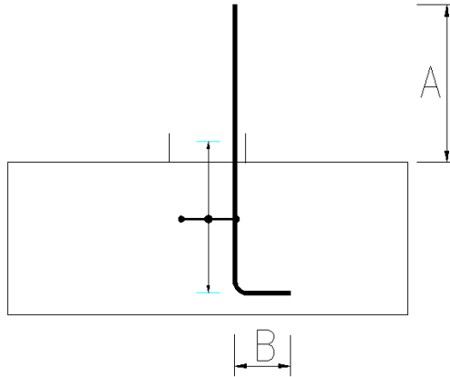
Figure 14.5.6:9 Starter Bar Dimensions
