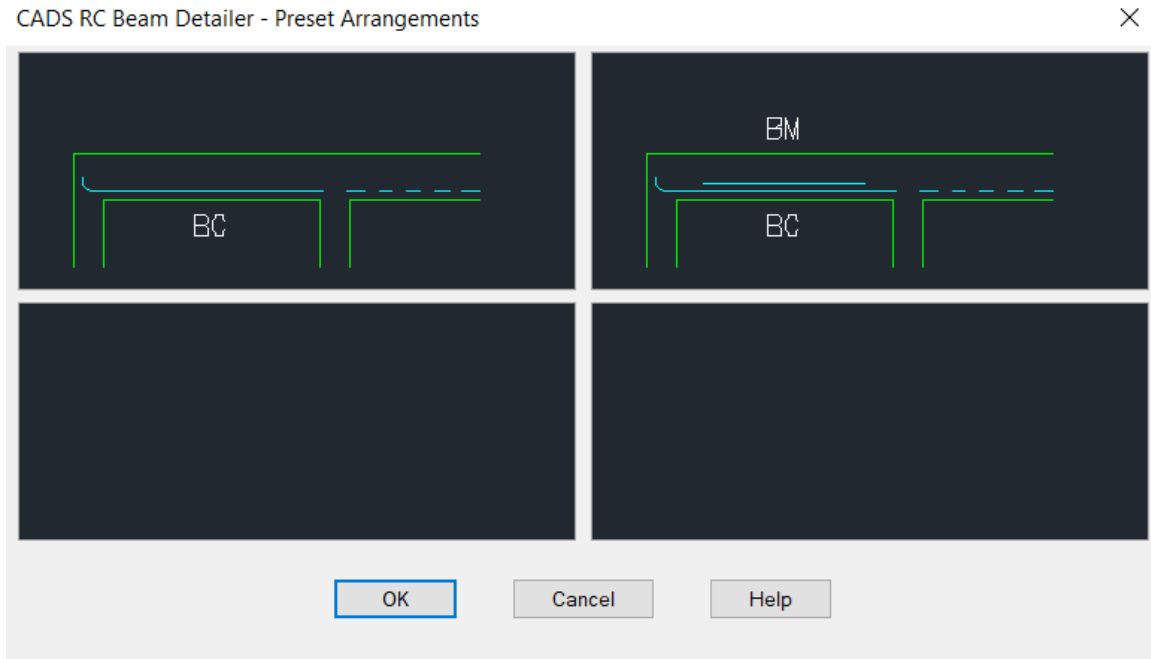
Figure 14.2.5:3 End Span Bottom Bar Pre-sets
