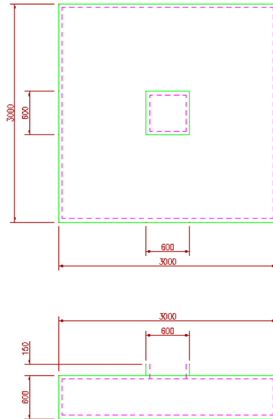
Figure 4.7.11:1 Pad Base Plan and Section created with CADS RC Outline Routines
