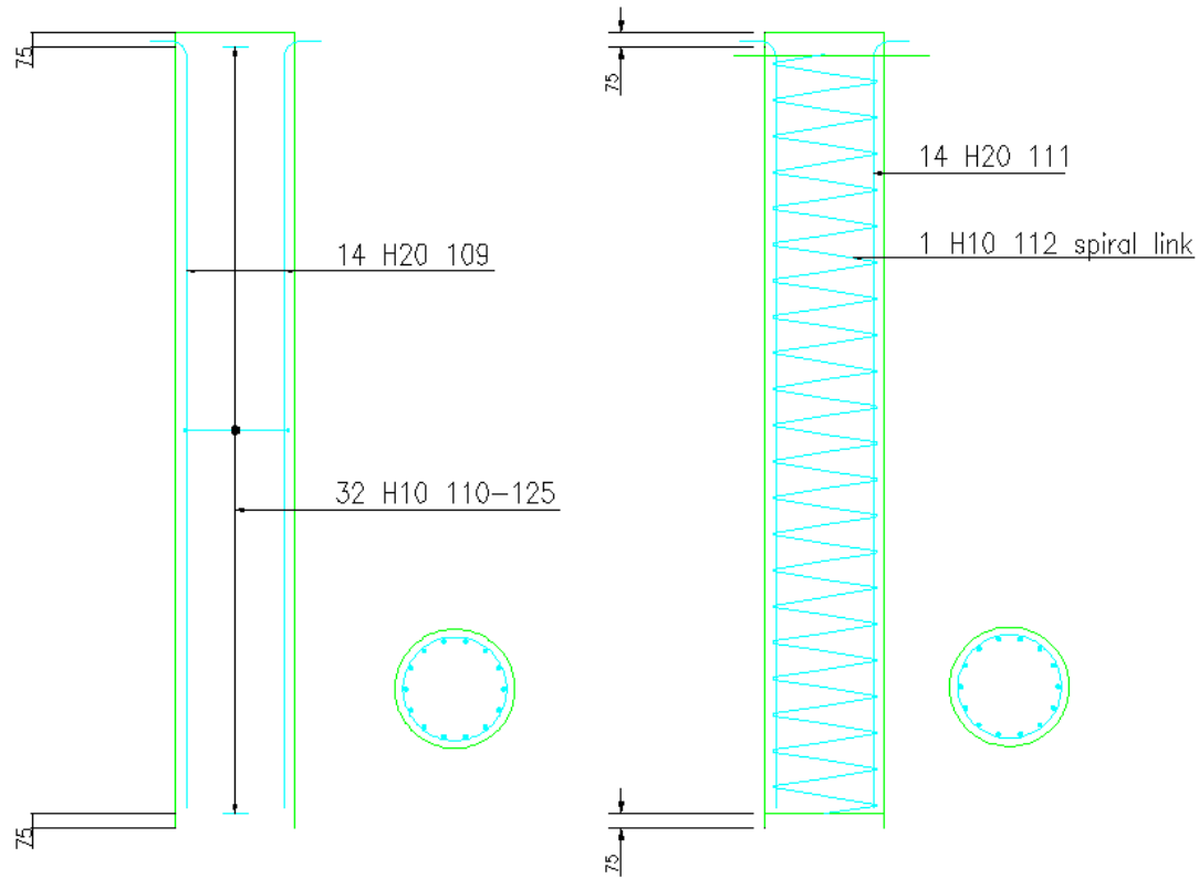
Figure 14.3.7:1 Typical Circular Column Elevations and Sections
