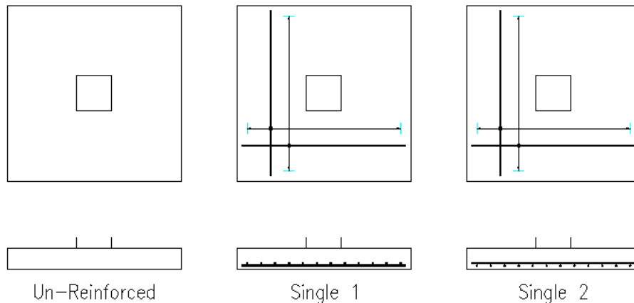
Figure 14.6.2:3 Typical Un-reinforced and Single Bar Arrangements
