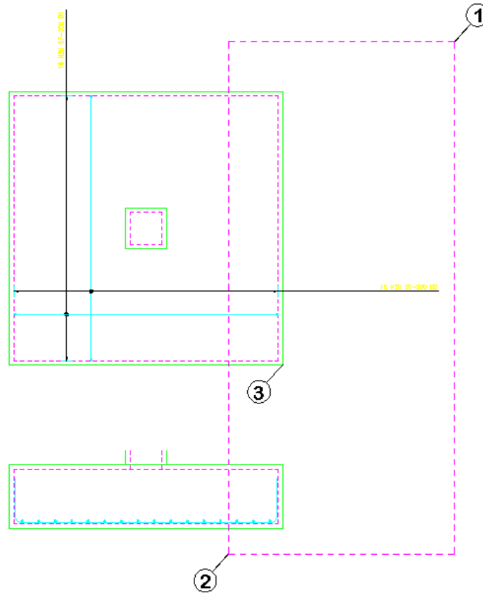
Figure 8.6.1:1 Pad Base before using Stretch Bar/Range
