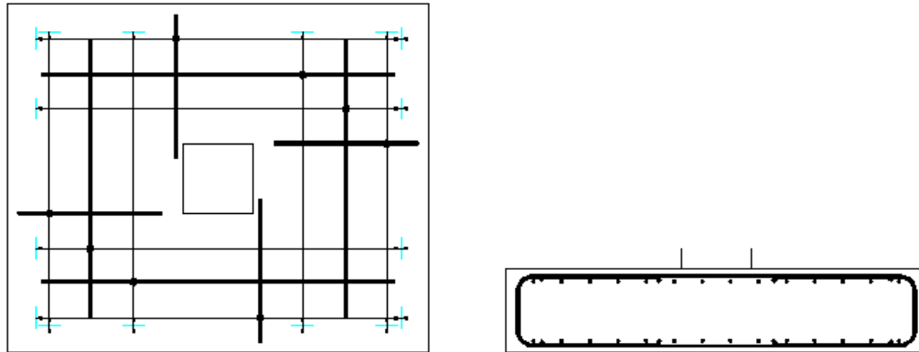
Figure 14.6.2:5 Typical Normal Bar Arrangement
