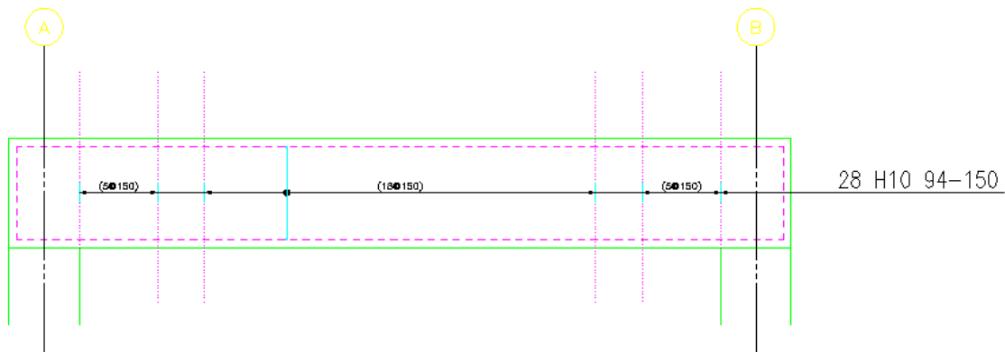
Figure 15.5.1:3 Single Indicator changed to a Single Multiple Pitch
