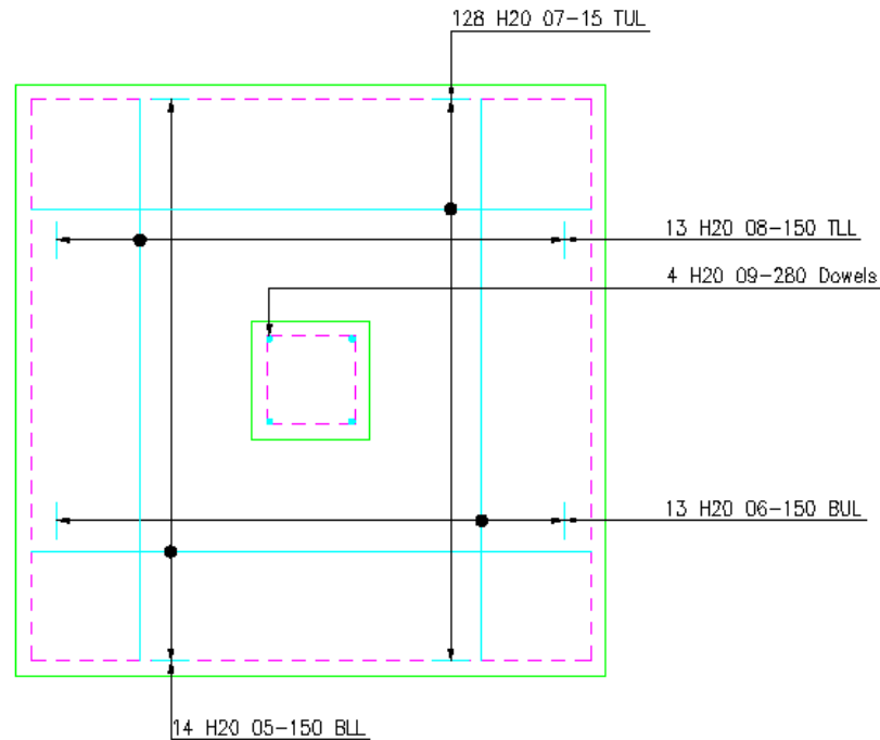
Figure 14.4.6:1 Typical Pad Footing Detail
