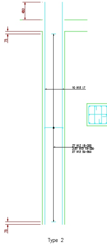
Figure 14.3.3:2 Column with column above
