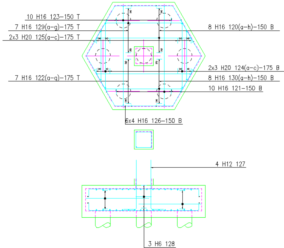
Figure 14.5 Typical Pile Cap Detail
