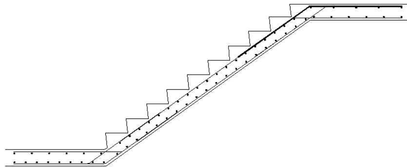
Figure 14.7.5:7 Bar Set 'G'
