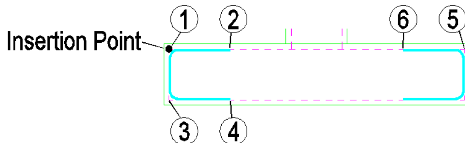
Figure 4.7.14:3 Insertion point and placing order Shape Code 21
