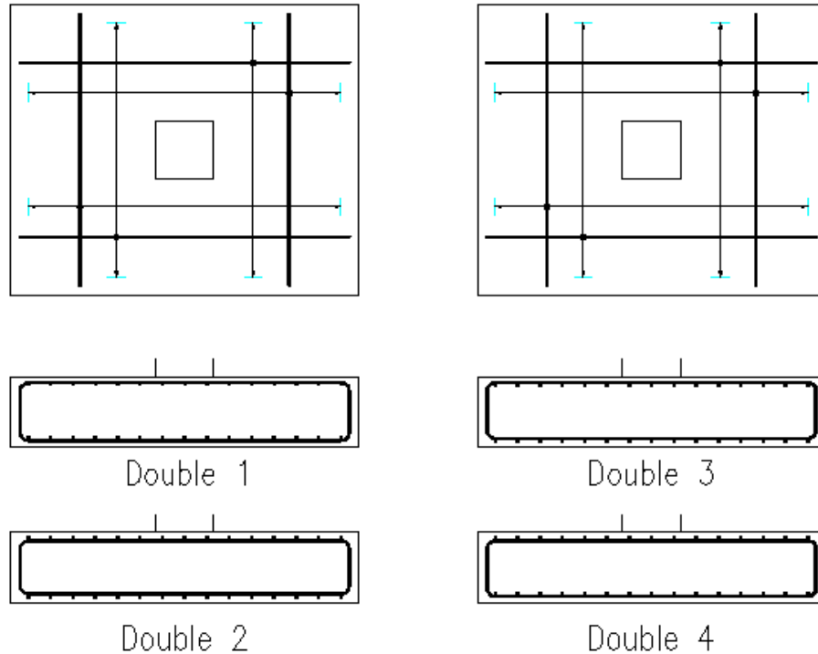
Figure 14.6.2:4 Typical Double Bar Arrangements
