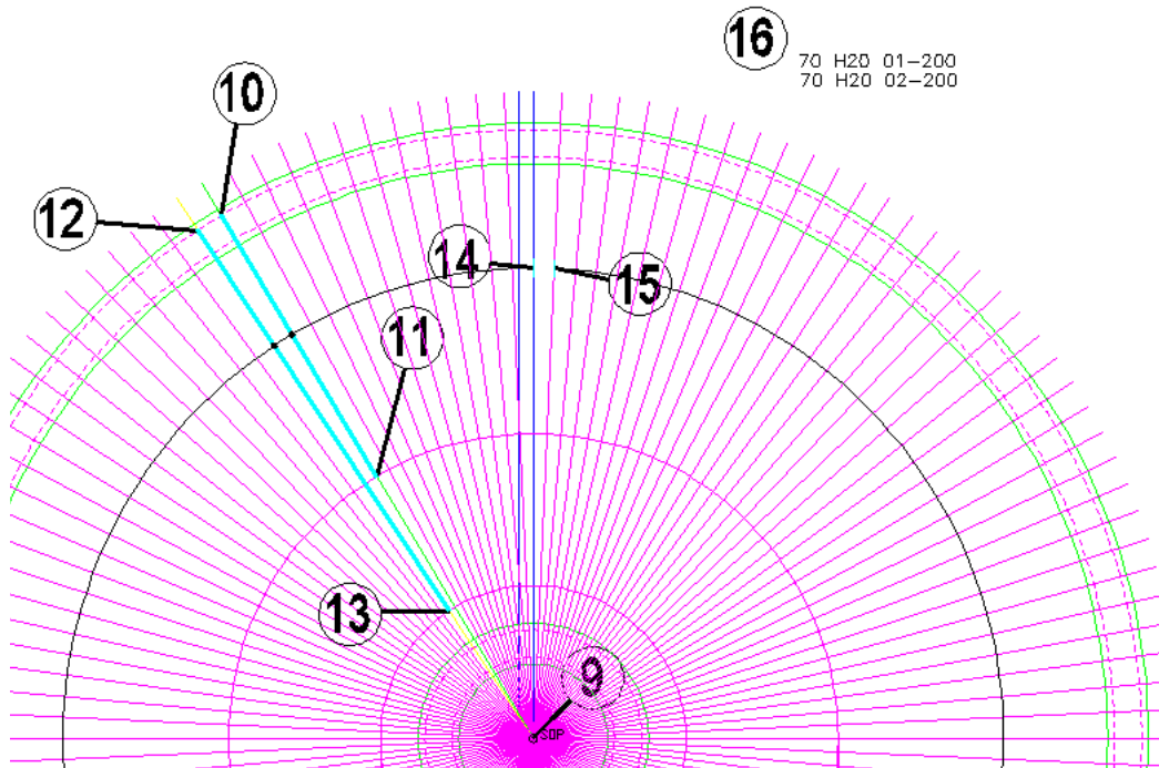
Figure 6.5.2.2 Adding an Alternate Radial Range to the Plan View of a Sump
