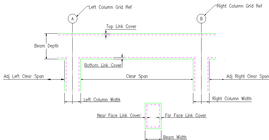
Figure 14.2.2:2 Beam Detailer Dimensions
