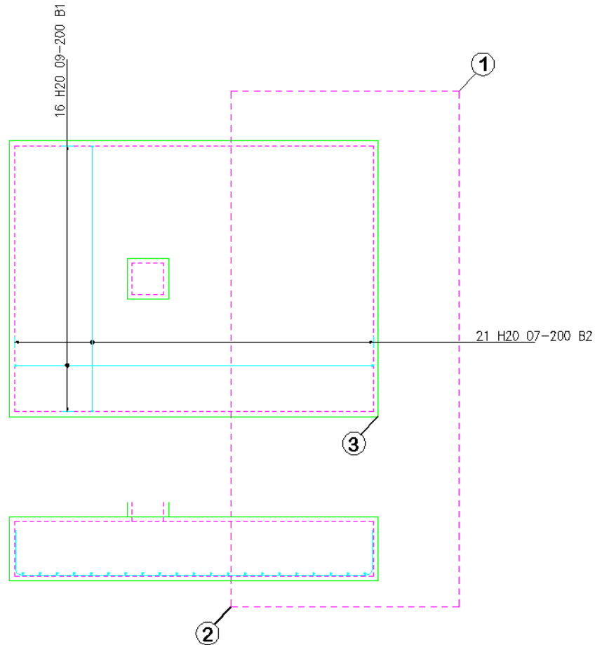
Figure 8.6.1:2 Pad Base after using Stretch Bar/Range
