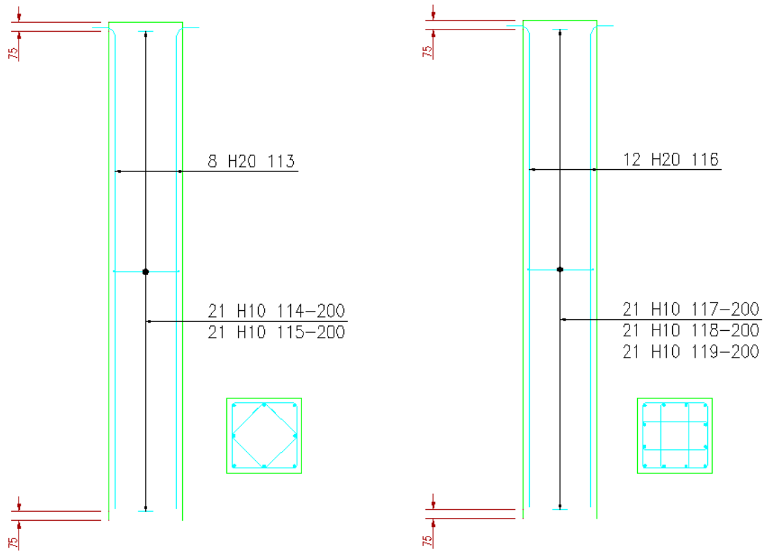
Figure 14.3.7:2 Typical Rectangular Column Elevations and Sections
