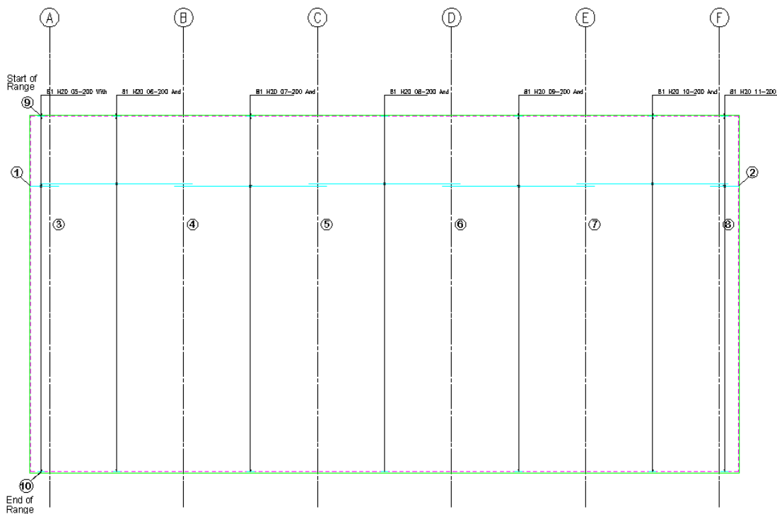
Figure 6.9.1:4 Adding OSL Bars and Ranges to a Floor Slab
