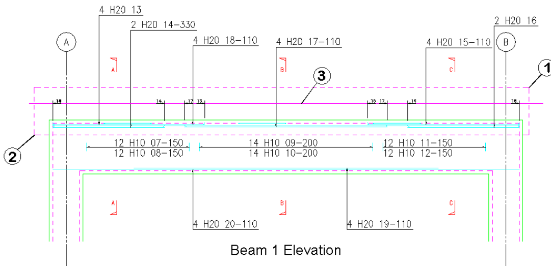
Figure 7.15.4:1 Tags added to Beam Elevation using Tag to a Line
