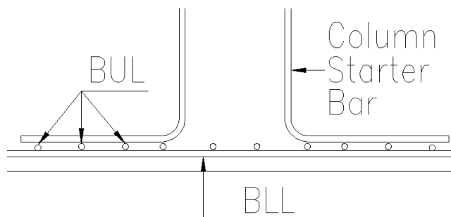
Figure 14.4.4:2 Column Dowel Hook detailed above BUL
