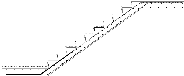
Figure 14.7.5:2 Bar Set 'B'
