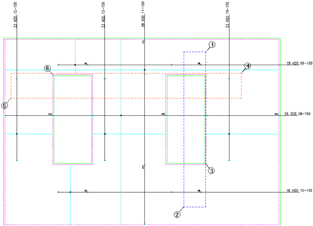
Figure 8.6.2:2 Slab with re-sized opening
