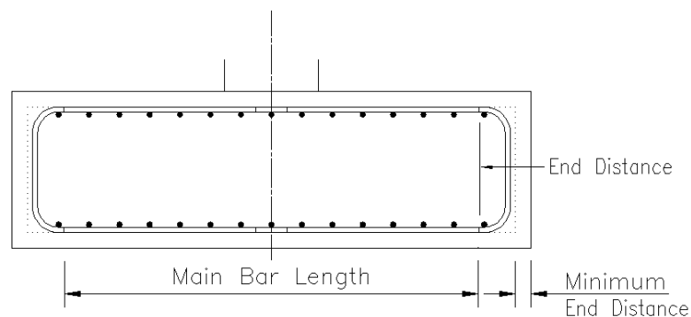
Figure 14.6.1:3 End Distance Information
