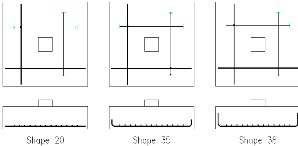
Figure 14.6.2:9 Single Longitudinal and Transverse Bar Shapes
