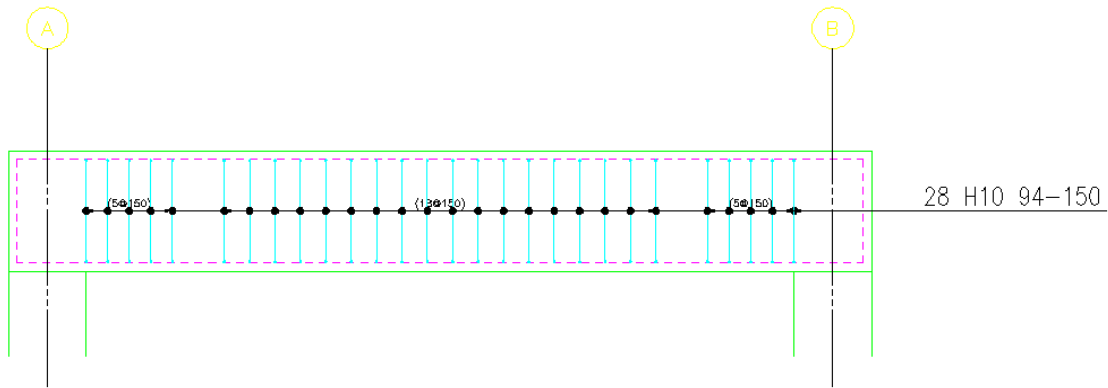
Figure 15.7.1:1 Multiple Pitch Range showing all bars
