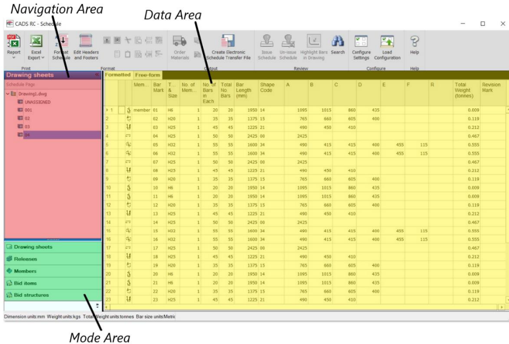
Figure 10.2:1 Schedule dialog
