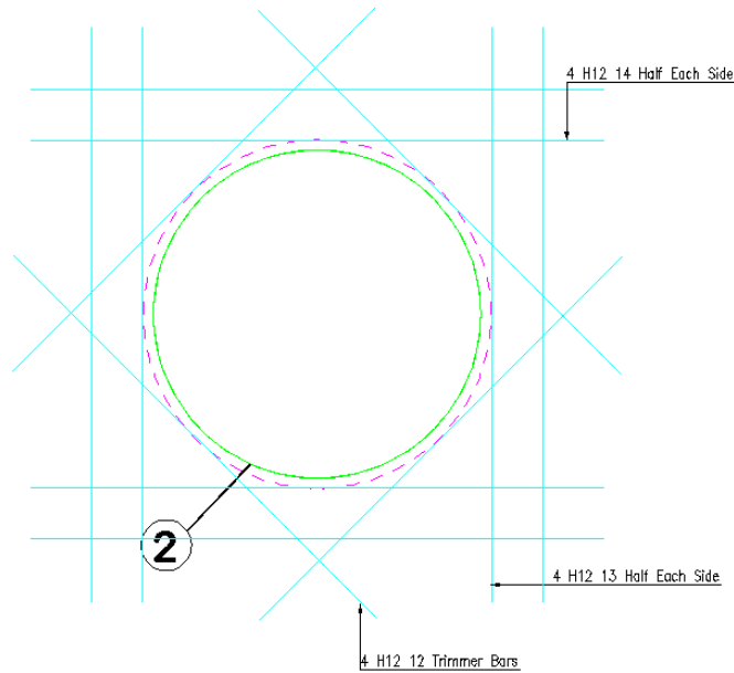
Figure 13.4.5:4 Trimmed Circular
