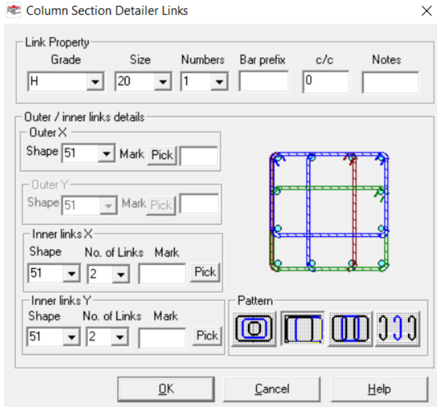
Figure 12.2.5:3 Links dialog
