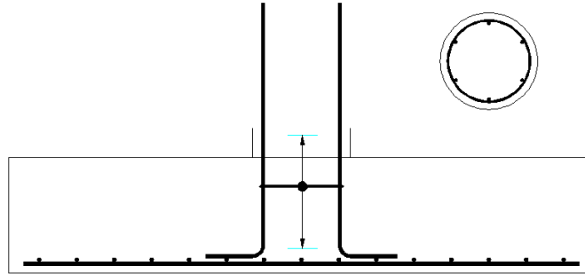
Figure 14.6.5:4 Typical Circular Column Starter Bar Detail
