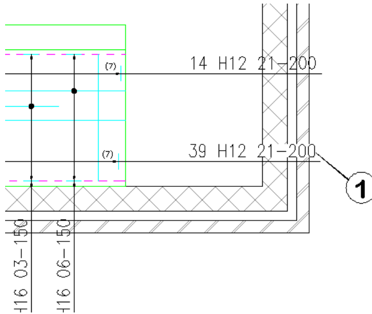
Figure 7.17:1 Masking of selected Bar Labels by using Mask Text
