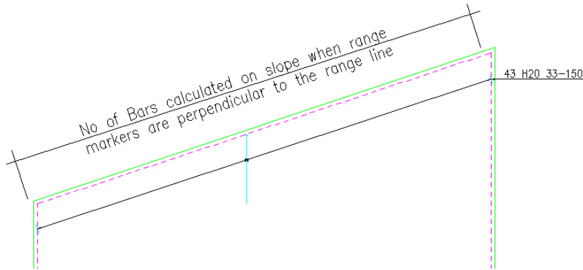
Figure 8.4.1:2 Range End Marker perpendicular to Range Line
