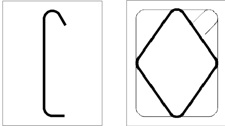
Figure 14.3.4:6 Inner Open Tie and Diamond Tie
