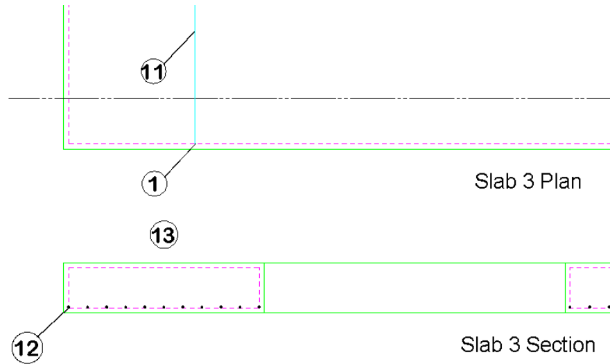
Figure 6.6.10:2 Adding a Staggered Fixed Pitch Run of Bars in Section to a Floor Slab
