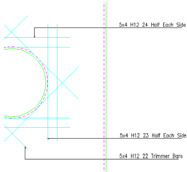
Figure 7.18:3 Bar Labels before Toggle Hidden Multipliers is switched on
