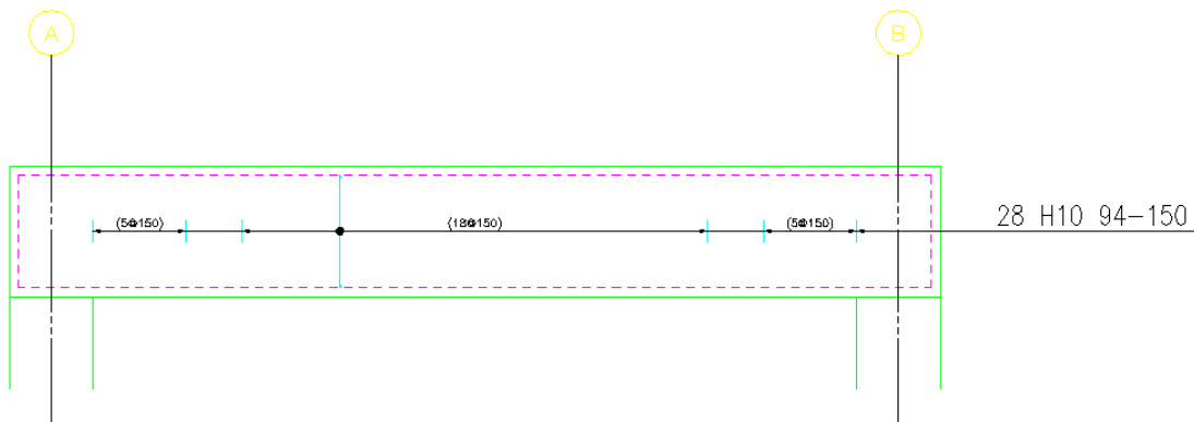
Figure 15.7.1 Range before showing all bars
