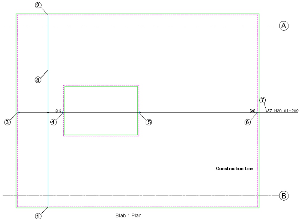
Figure 6.6.2:1 Adding a Single Fixed Pitch Range to a Floor Slab
