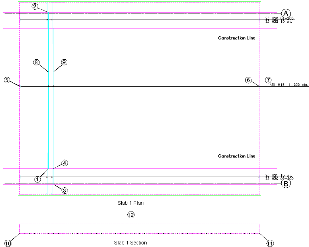
Figure 6.3.10:1 Adding a Staggered Range to a Floor Slab
