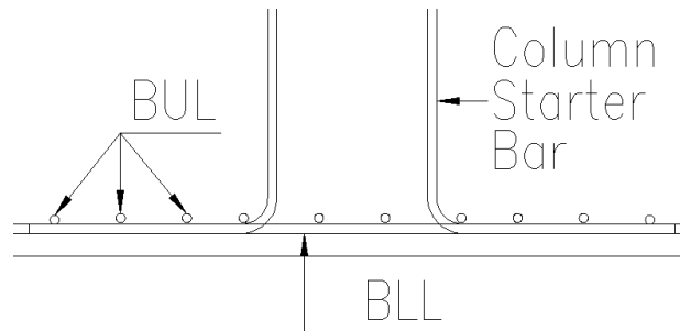
Figure 14.4.4:1 Column Dowel Hook detailed in BLL
