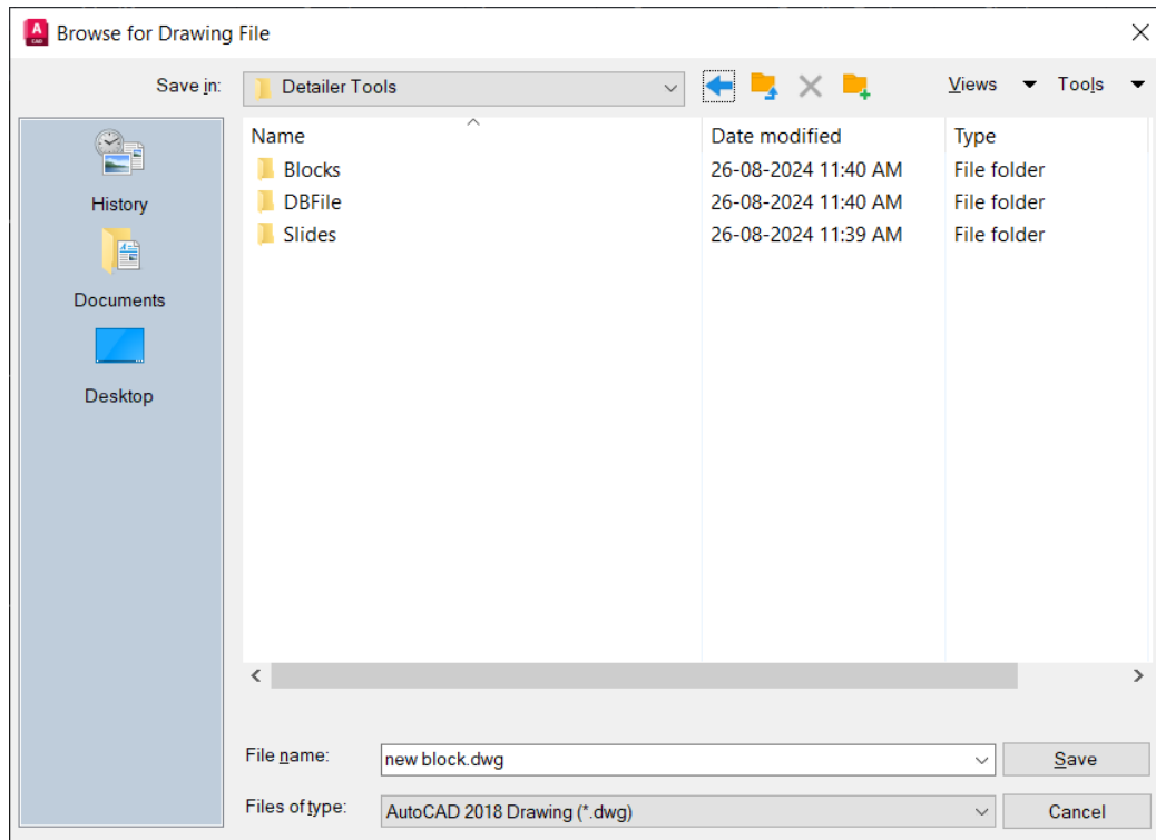
Figure 8.12.2:1 Wblock dialog
