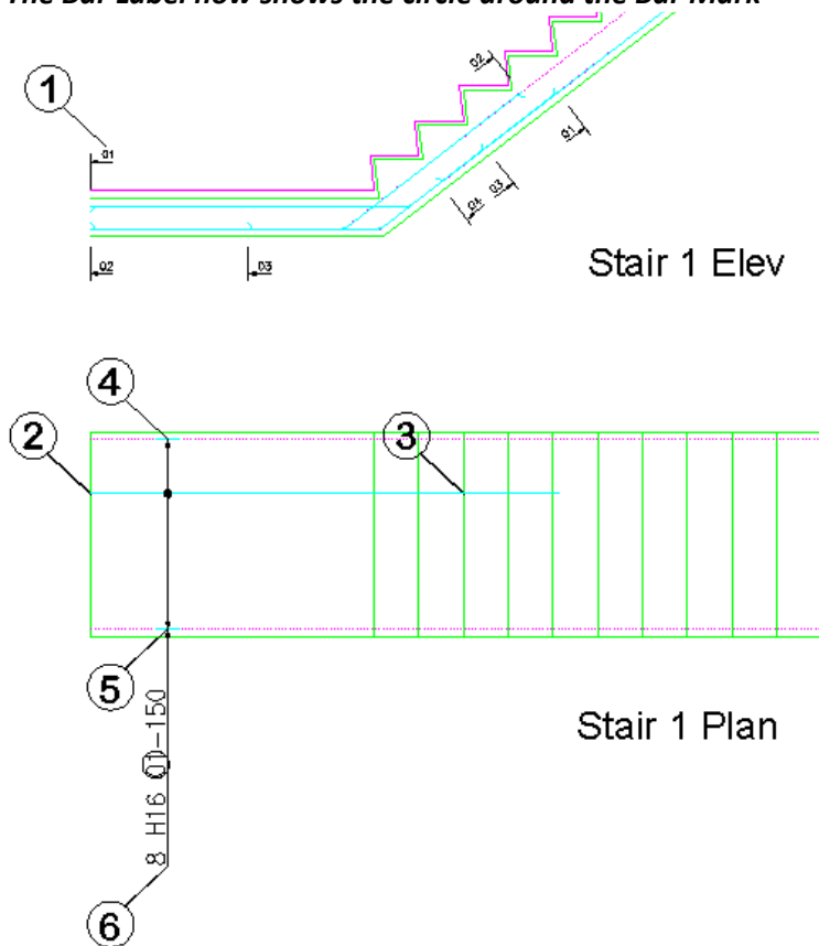
Figure 7.12.1:1 Bar Label for cranked bars showing new format
