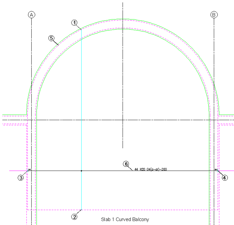
Figure 6.7.11:1 Adding a Varying Taper Range to a curved balcony
