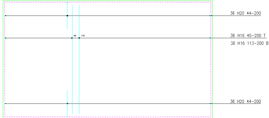
Figure 15.6.2:1 Stretched detail
