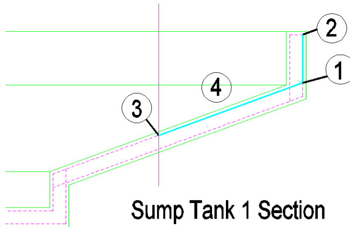
Figure 6.3.12:1 Adding Shape Code 15 to a Section through a sump tank
